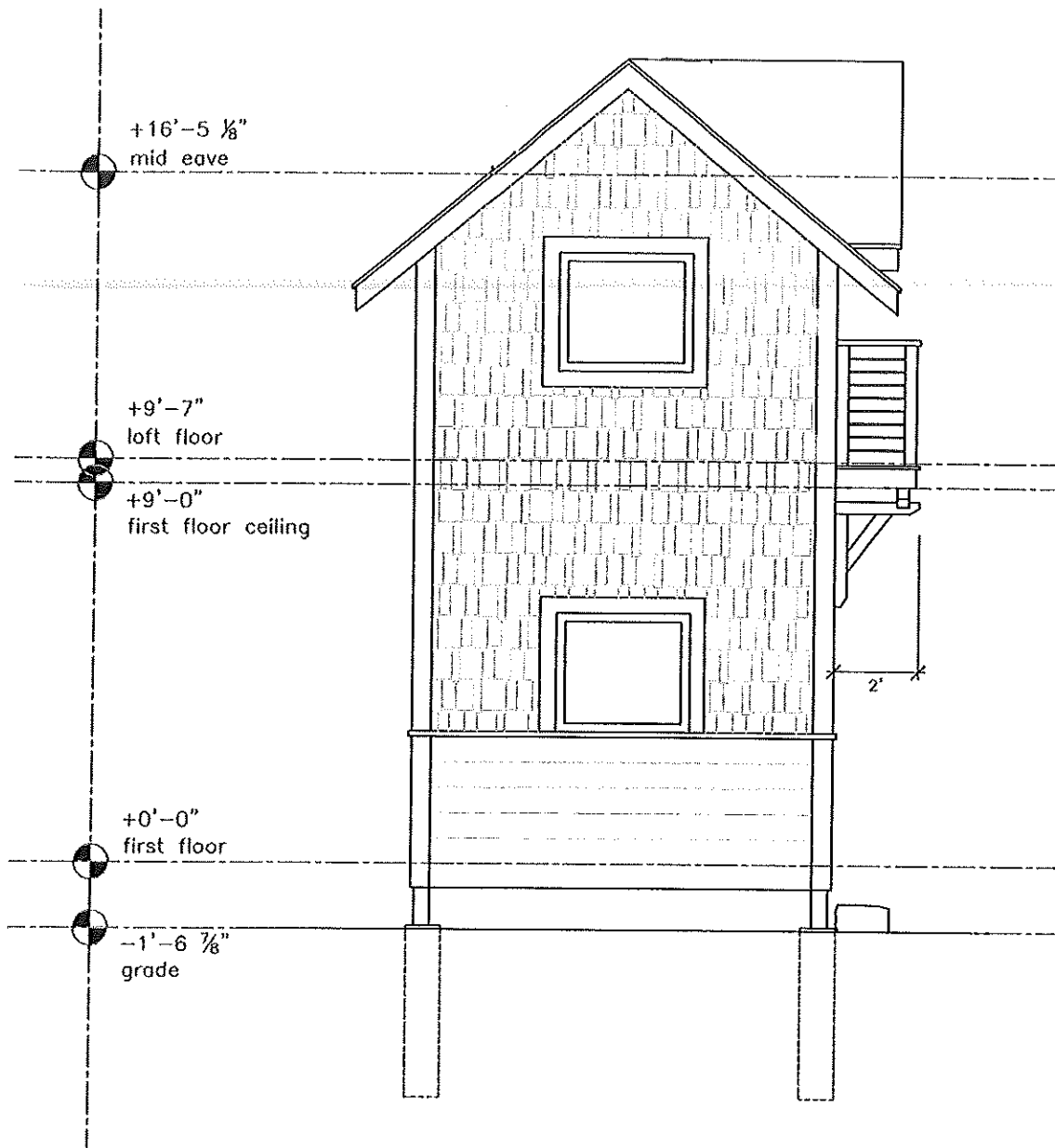
A West Elevation \frac{1}{4}'' = 1'-0''
