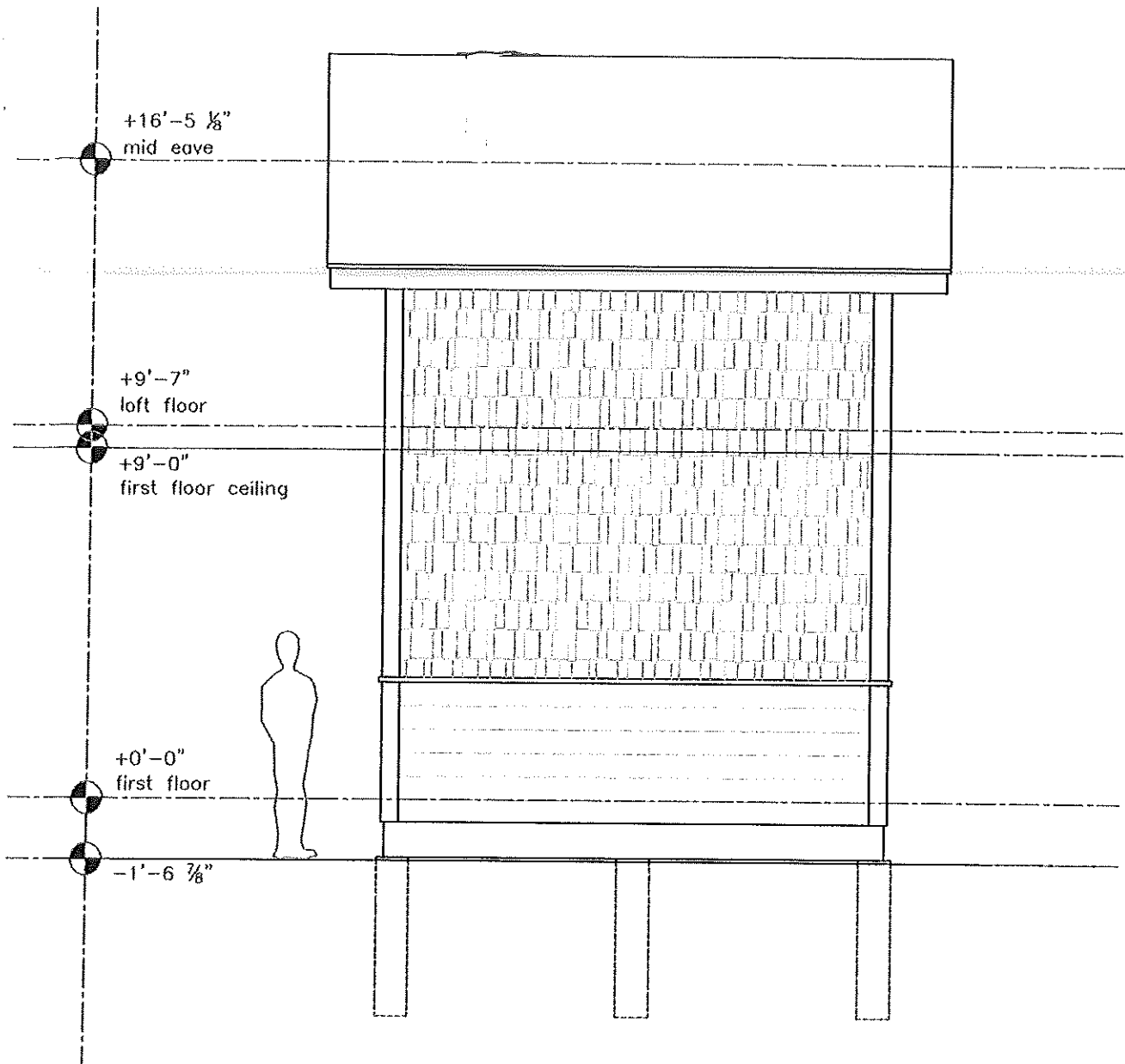
A North Elevation \frac{1}{4}" = 1'-0"
