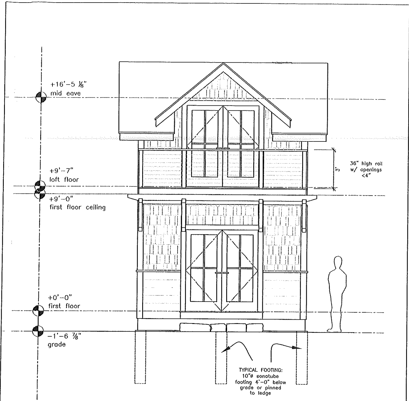
A South Elevation \frac{1}{4}'' = 1' - 0''
