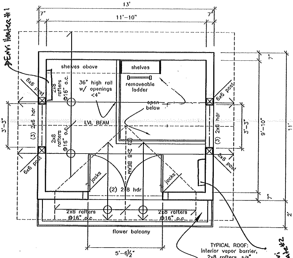
(B) Loft Plan/Roof Framing \frac{1}{4}'' = 1'-0''
