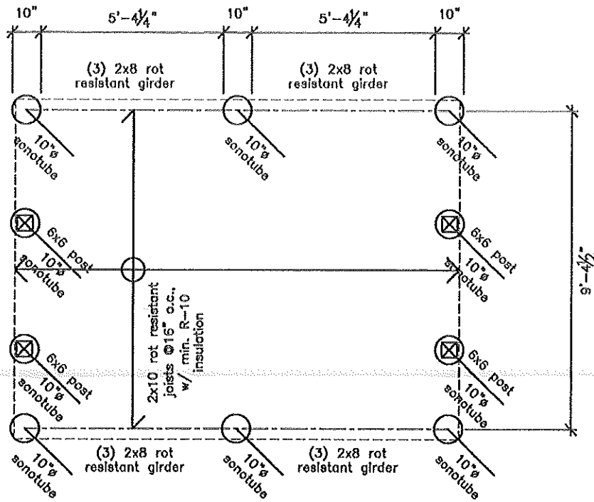
(A) Foundation Plan/First Floor Framing 1/4" = 1'-0"
