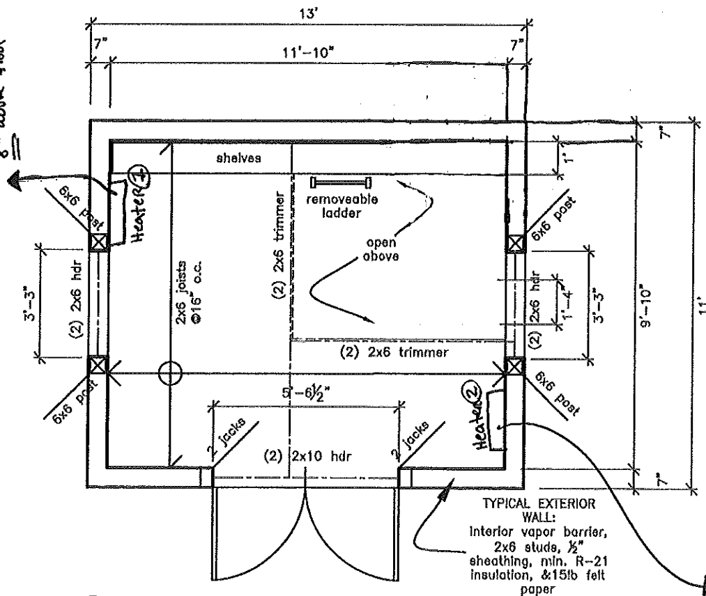
(B) First Floor Plan/Second Floor Framing 1/4" = 1'-0"
