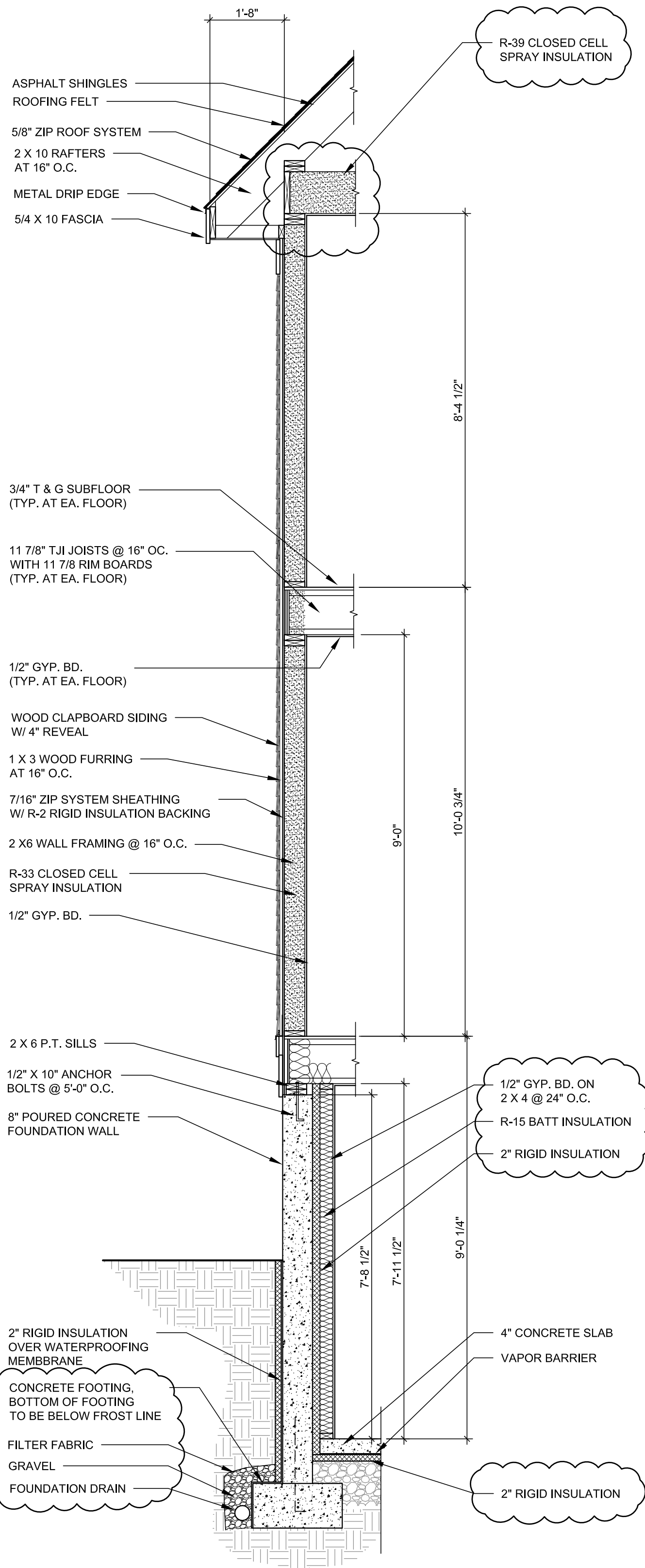
5 WALL SECTION 1/2" = 1'-0"
