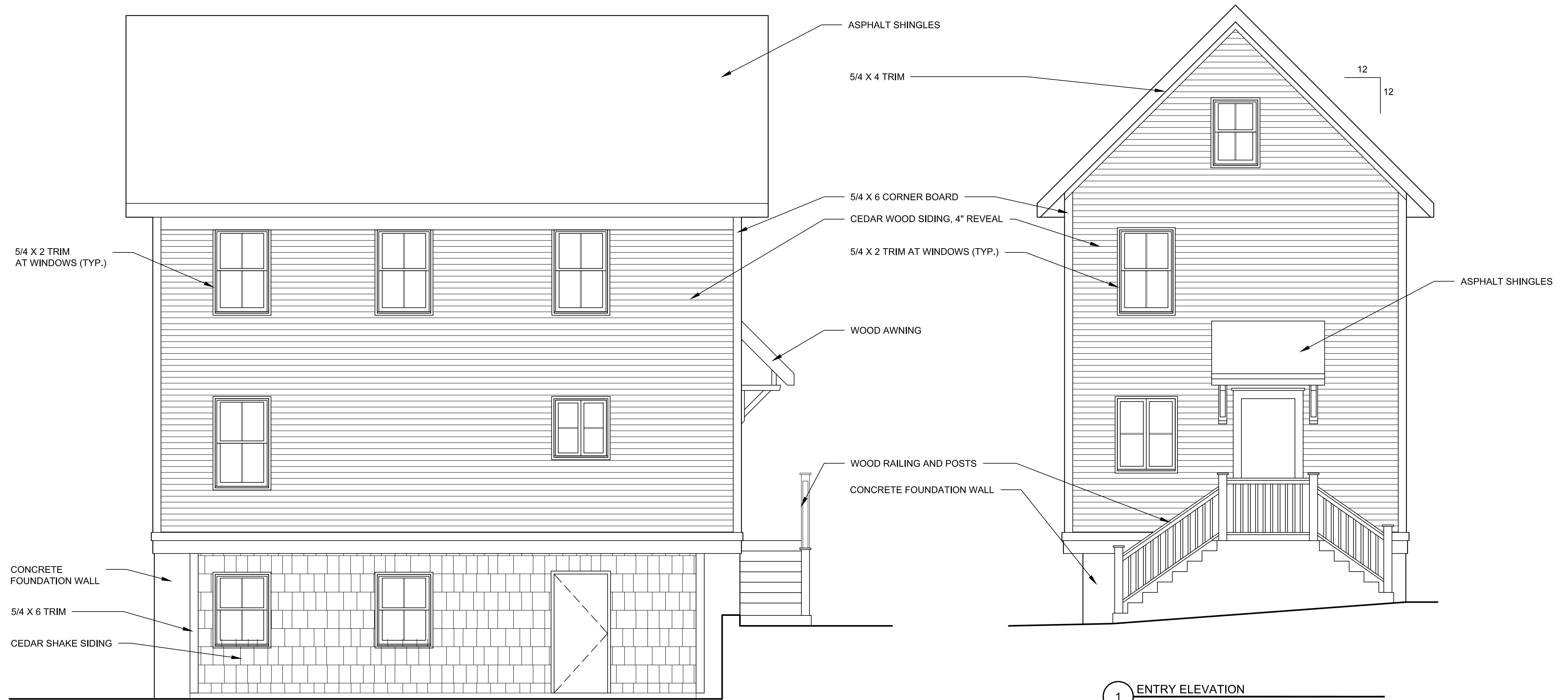
1 ENTRY ELEVATION 1/4" = 1'-0"
