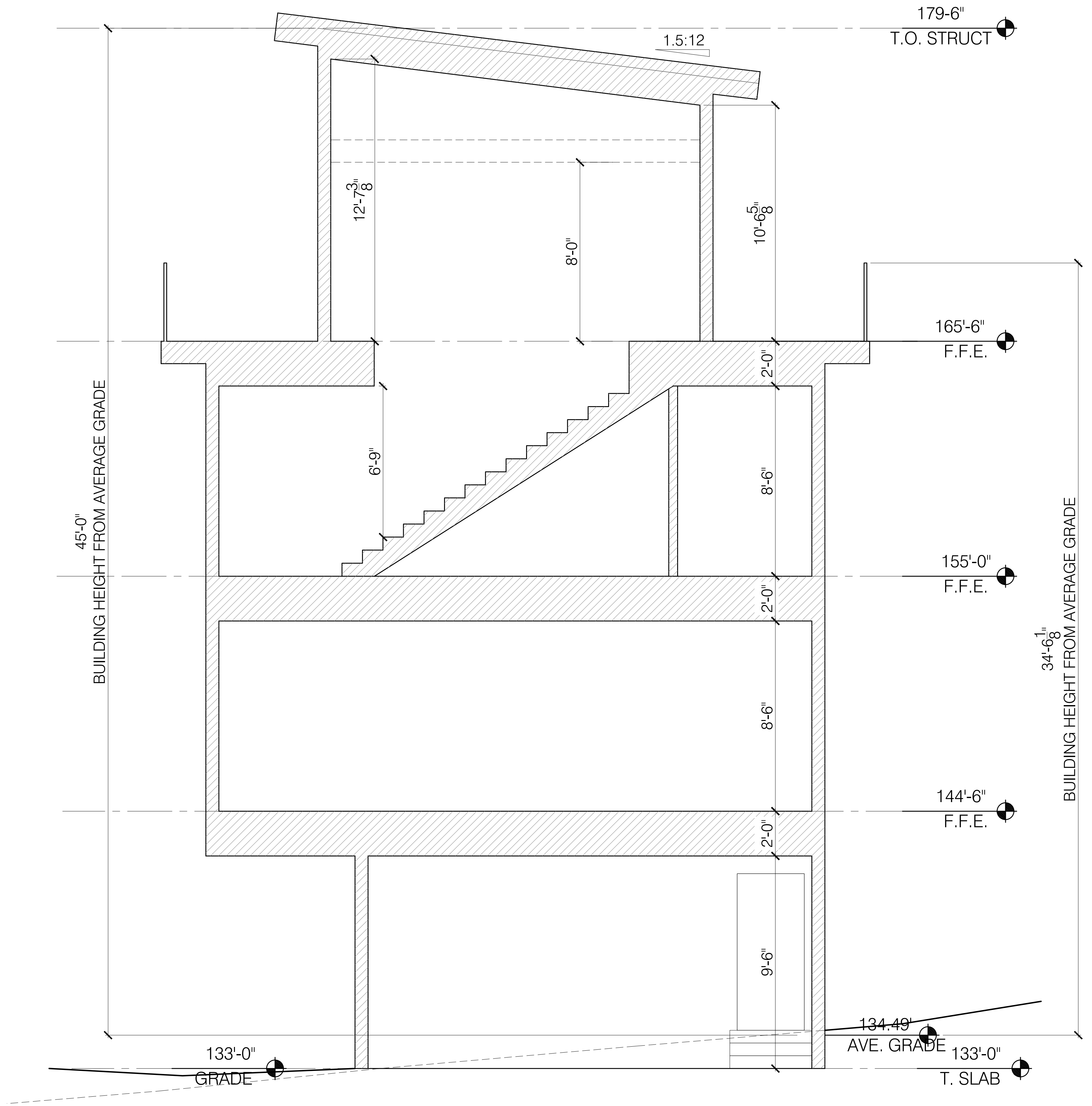
1 BUILDING SECTION 0 3'-0" SCALE: 3/8" = 1'-0"
