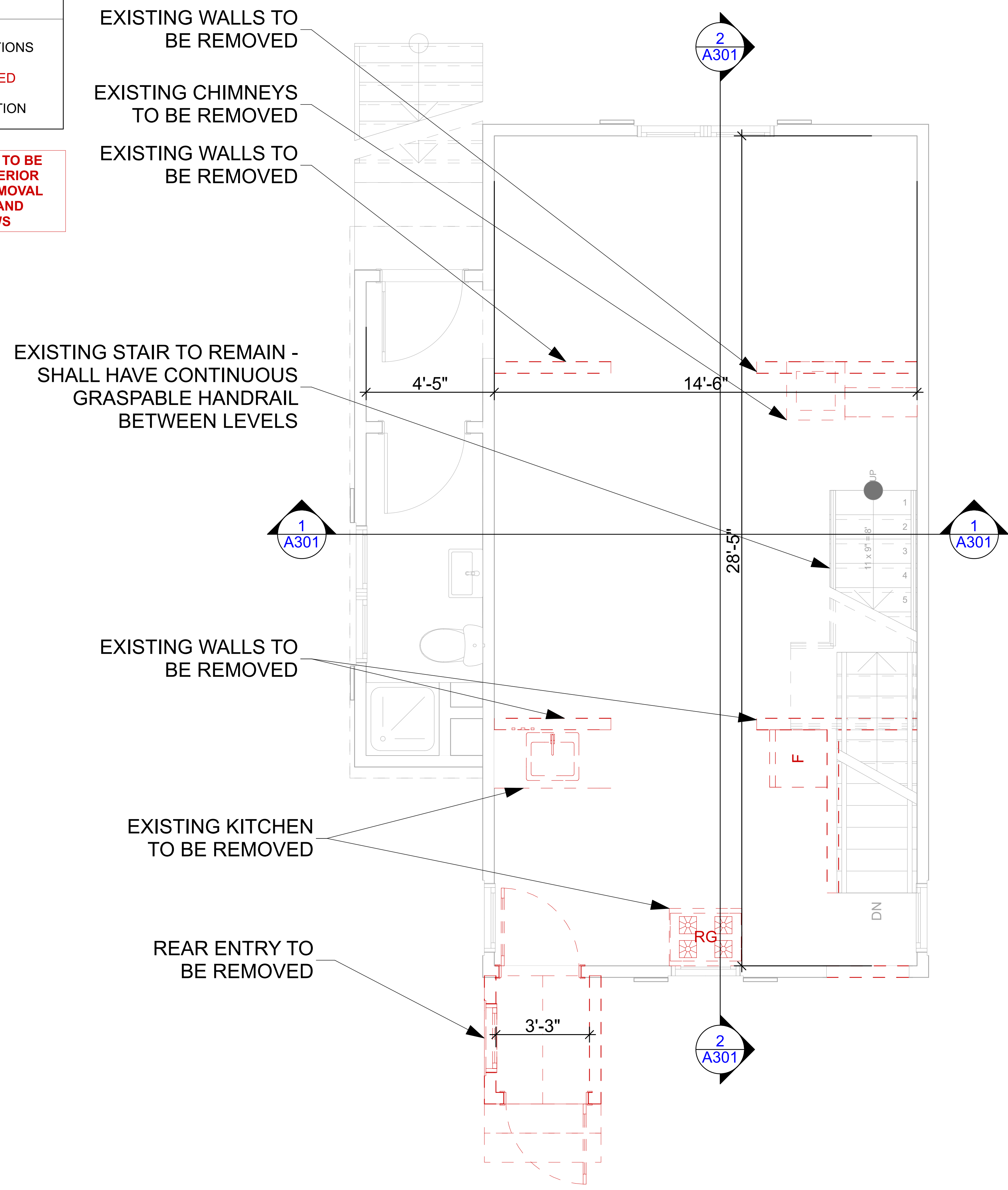
2 1ST FLOOR - TO BE DEMOLISHED SCALE: 1/2" = 1'-0"
