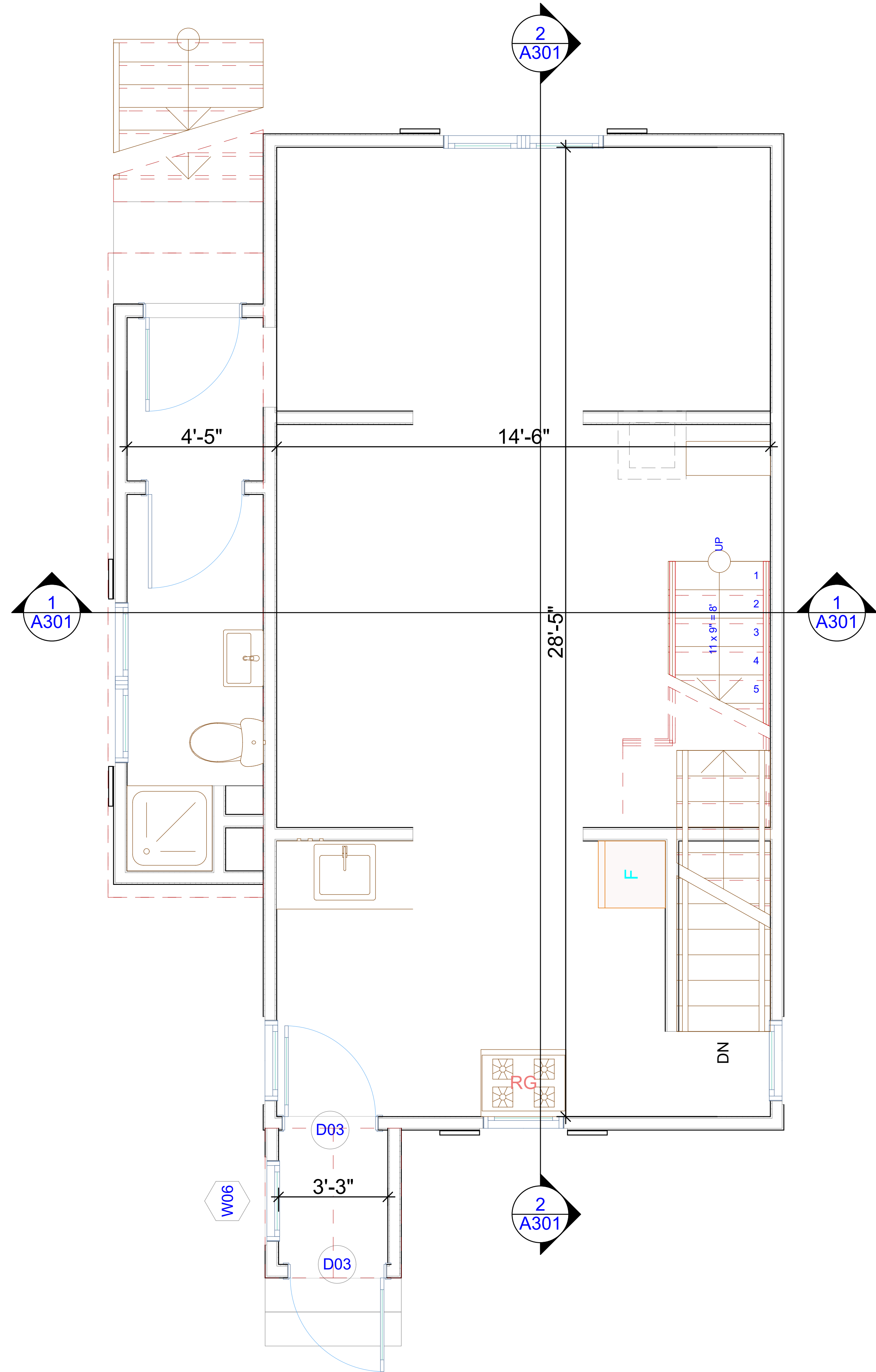
2 1ST FLOOR - EXISTING SCALE: 1/2" = 1'-0"
