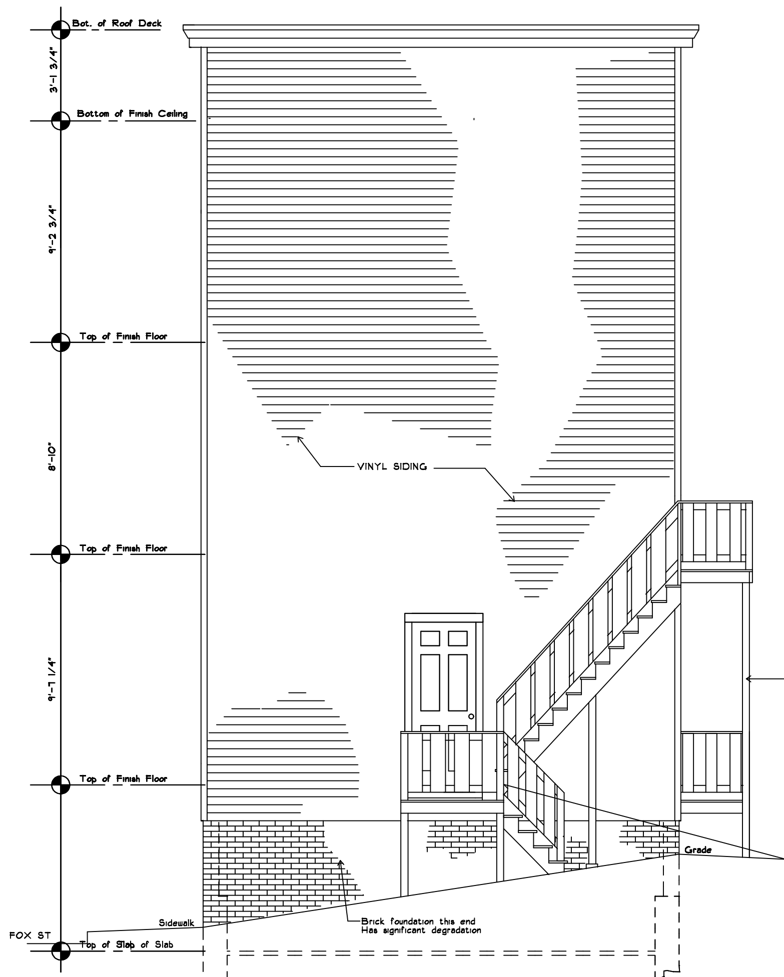
42 Greenleaf Street South Elevation 1/4"=1'-0"
