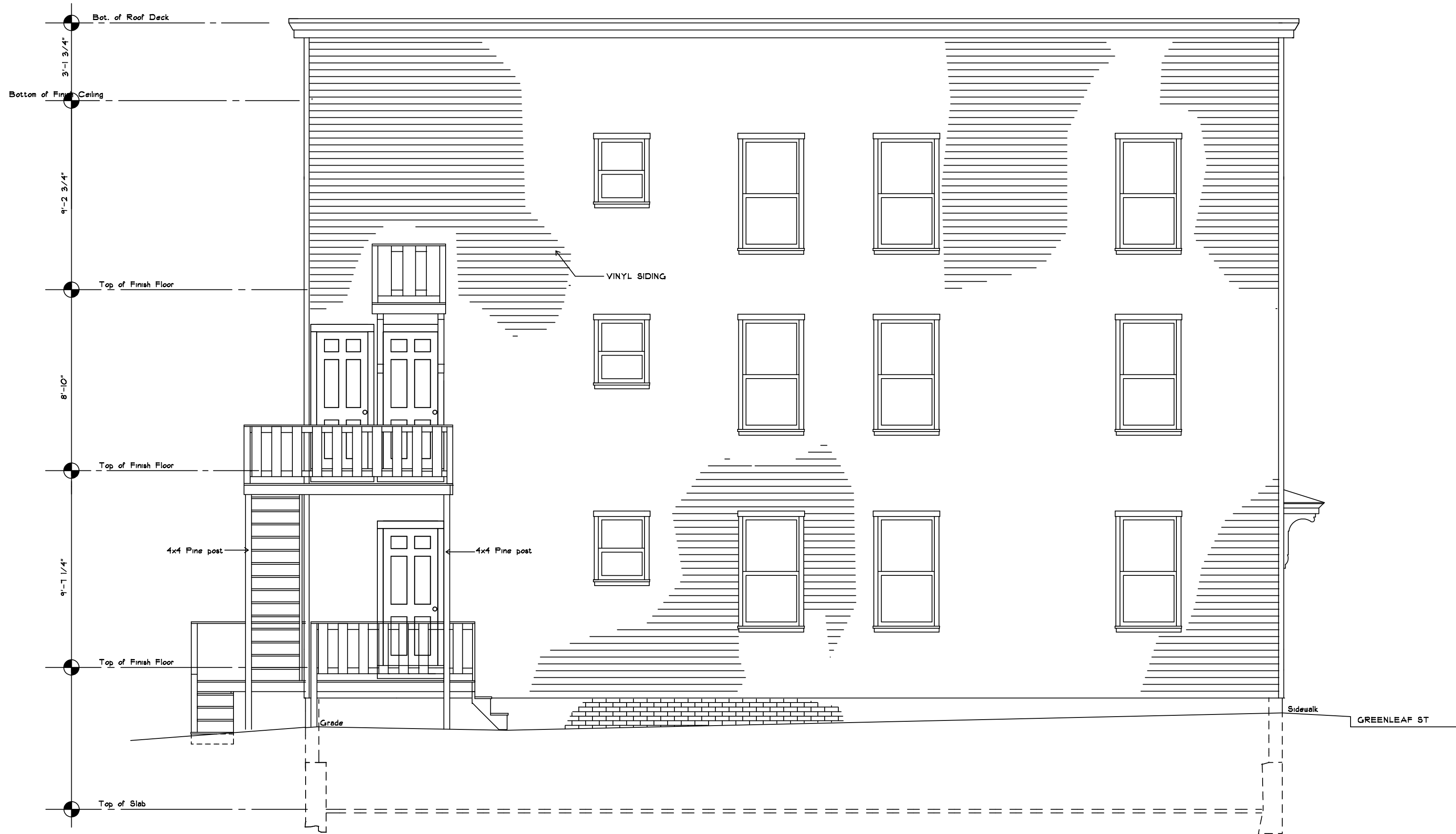
42 Greenleaf Street East Elevation 1/4"=1'-0"
