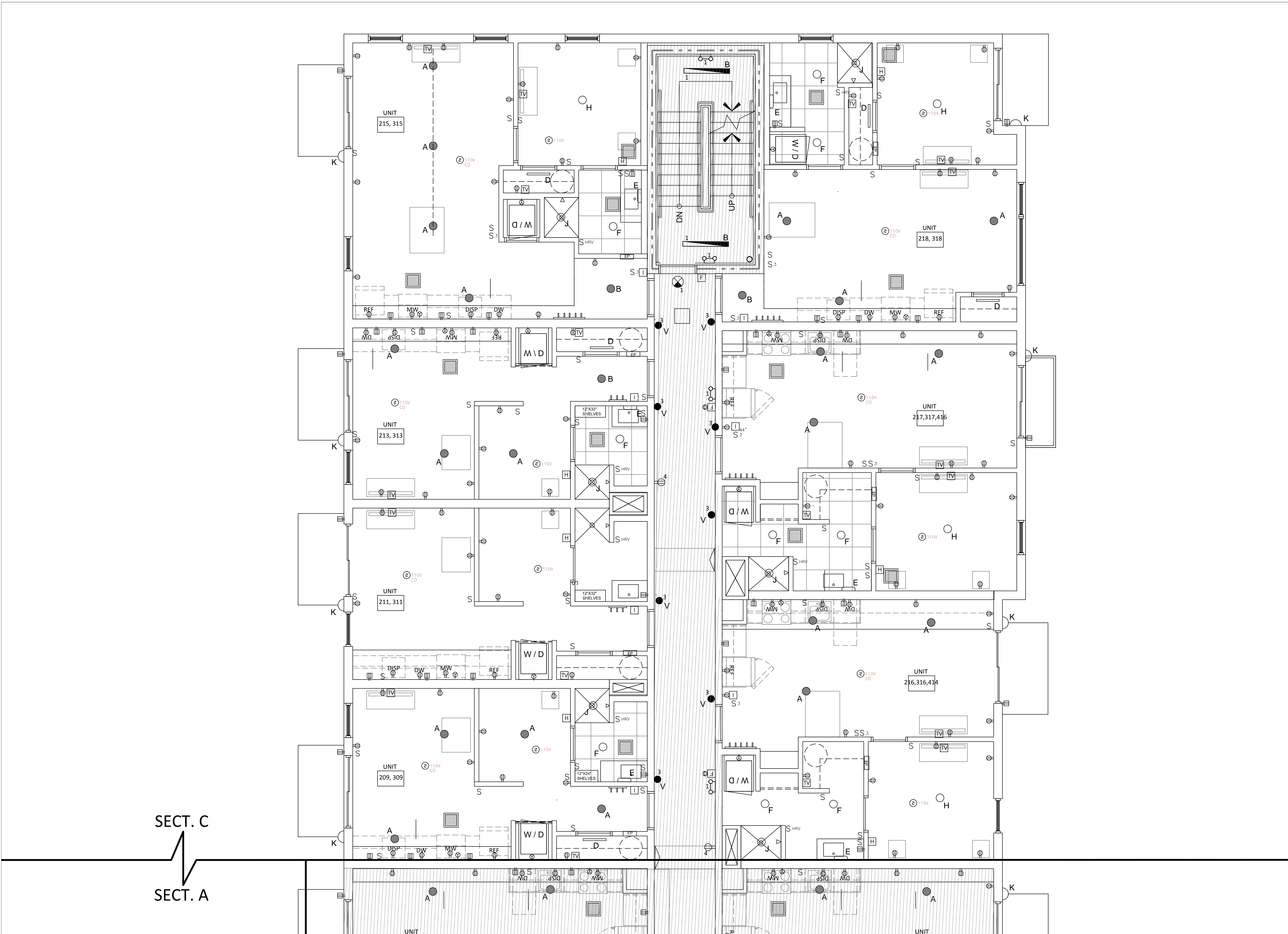
UNIT LAYOUTS TYPICAL - 2ND, 3RD, 4TH - SECTION C
