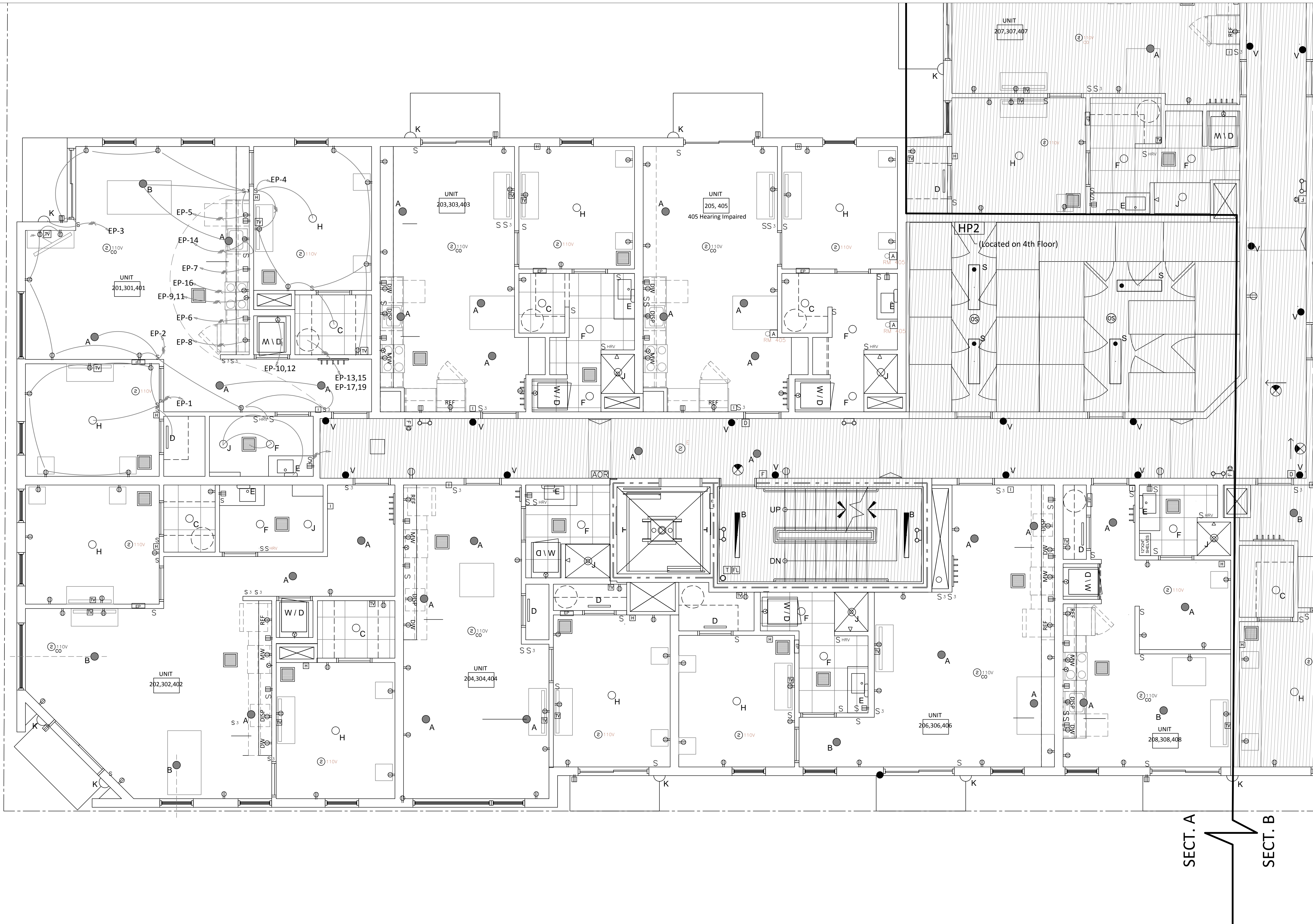
UNIT LAYOUTS TYPICAL - 2ND, 3RD, 4TH - SECTION A
