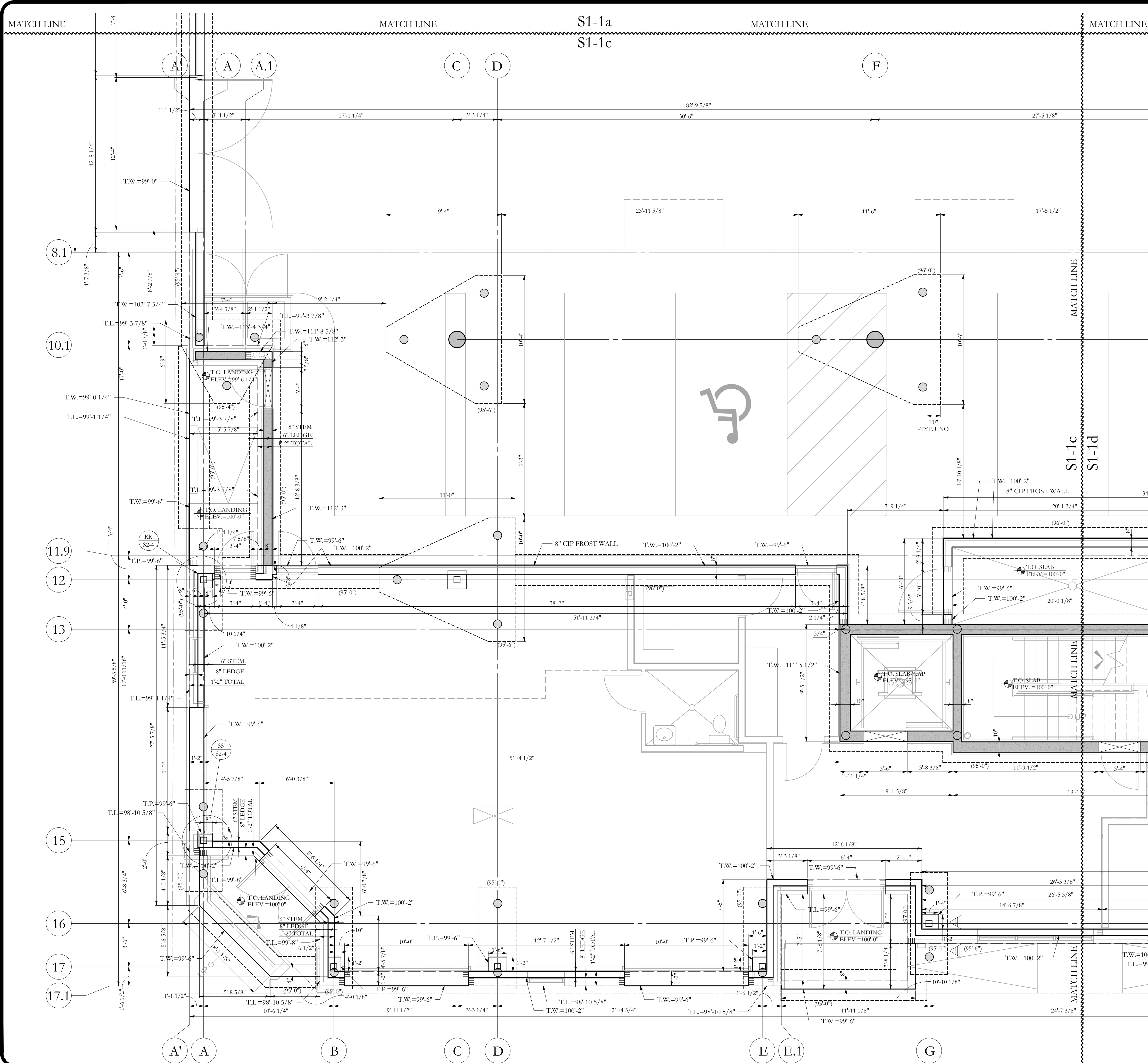
FOUNDATION DIMENSION PLAN C
