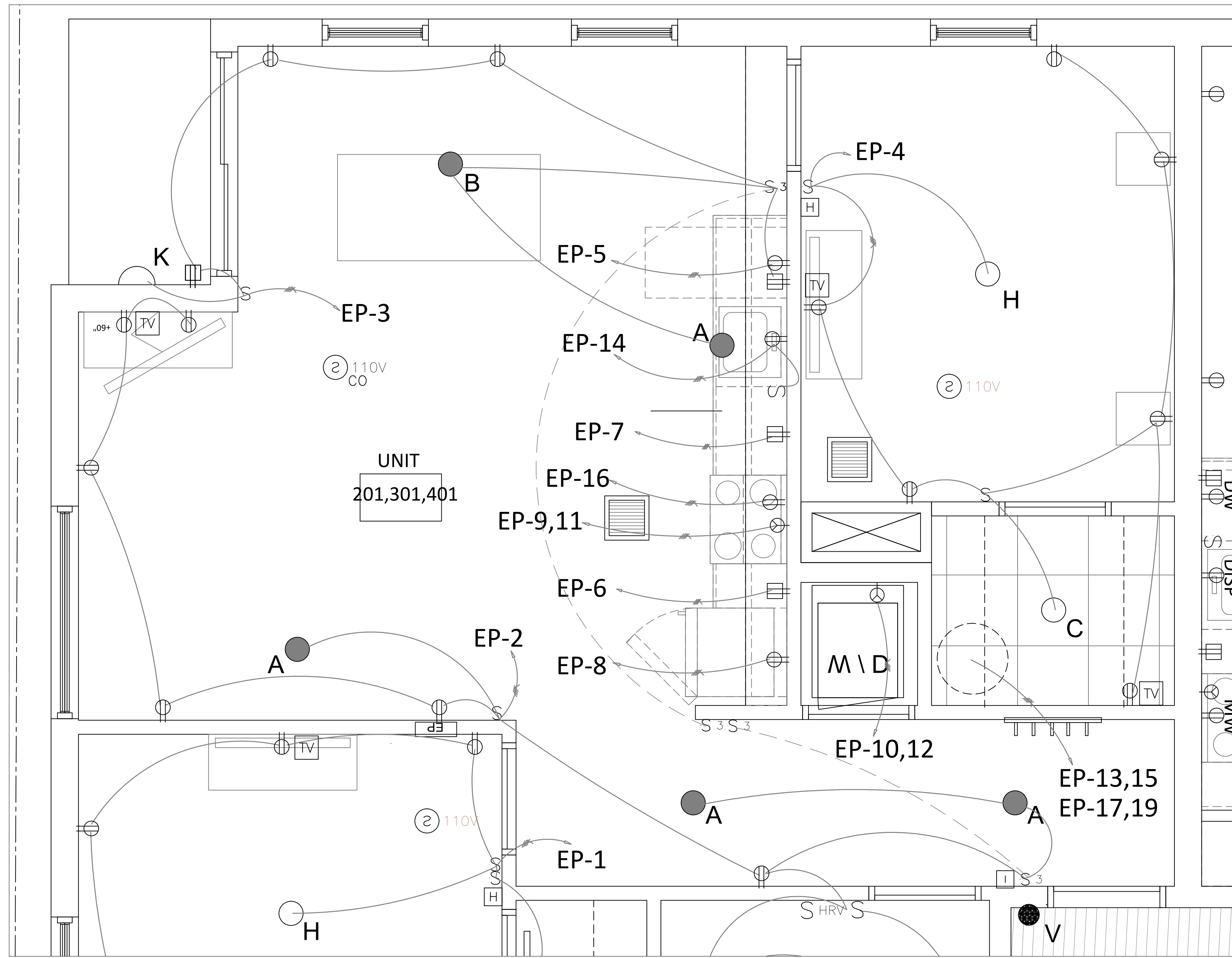
SAMPLE UNIT CIRCUITING - 210, 310, 410
