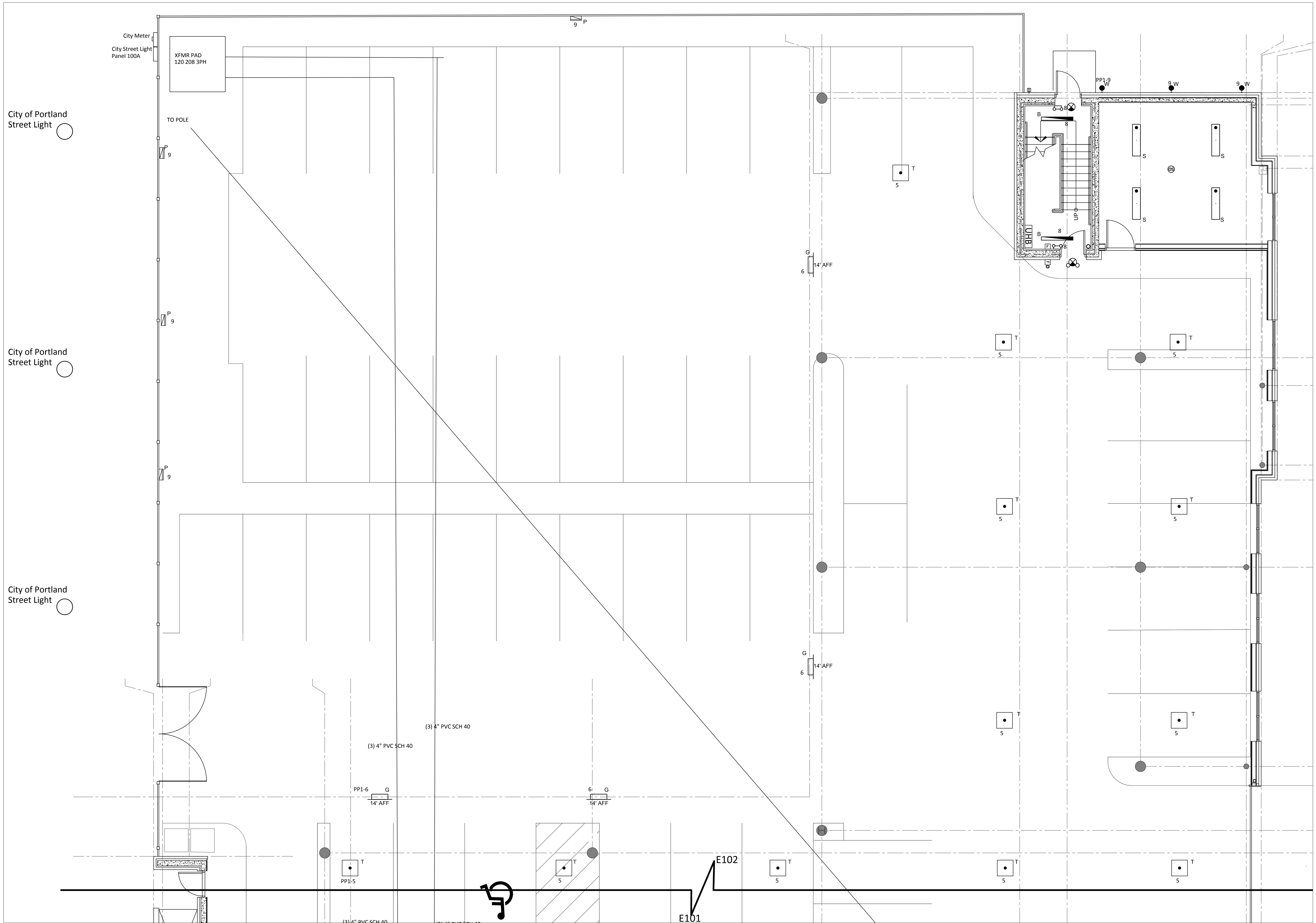
FIRST FLOOR - SITE LIGHTING
