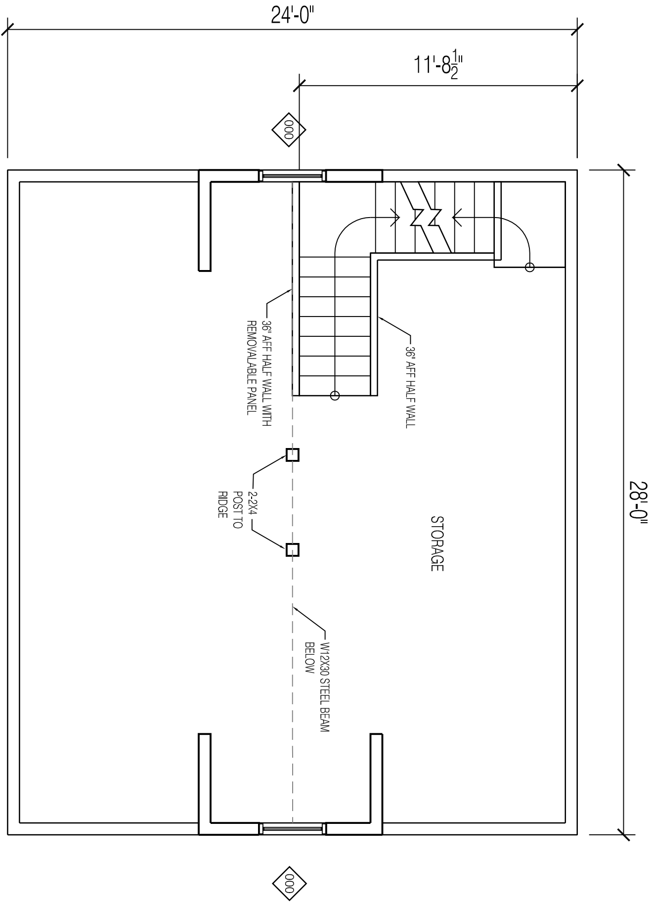
GARAGE SECOND FLOOR 1/4" = 1'-0"
