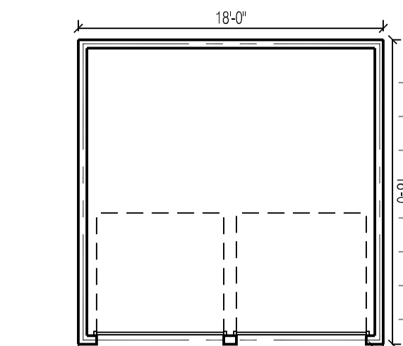
FIRST FLOOR EXISTING PLAN 1/8" = 1'-0"
