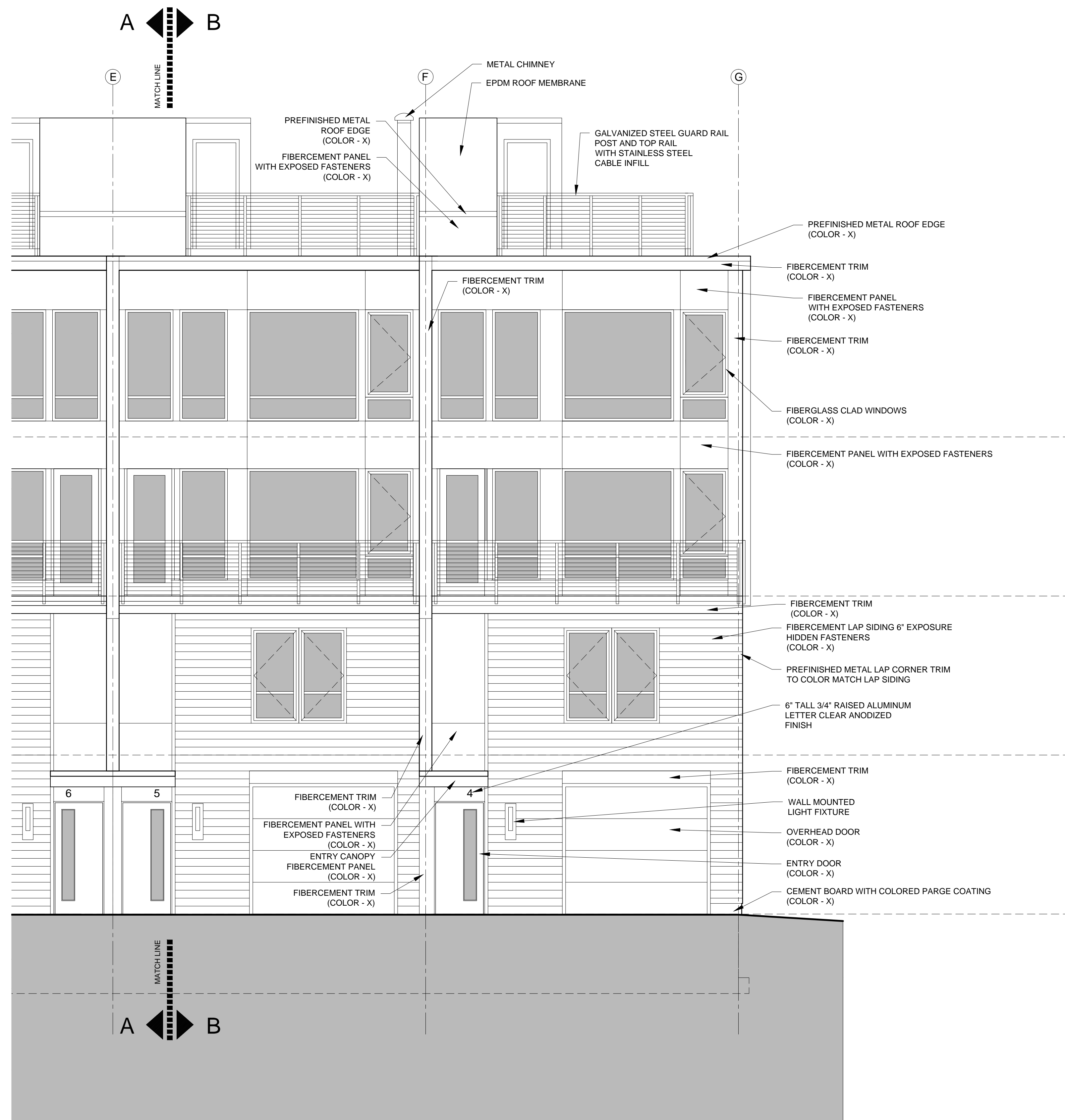
1 SOUTH ELEVATION - PART B 1/4"=1'-0"
