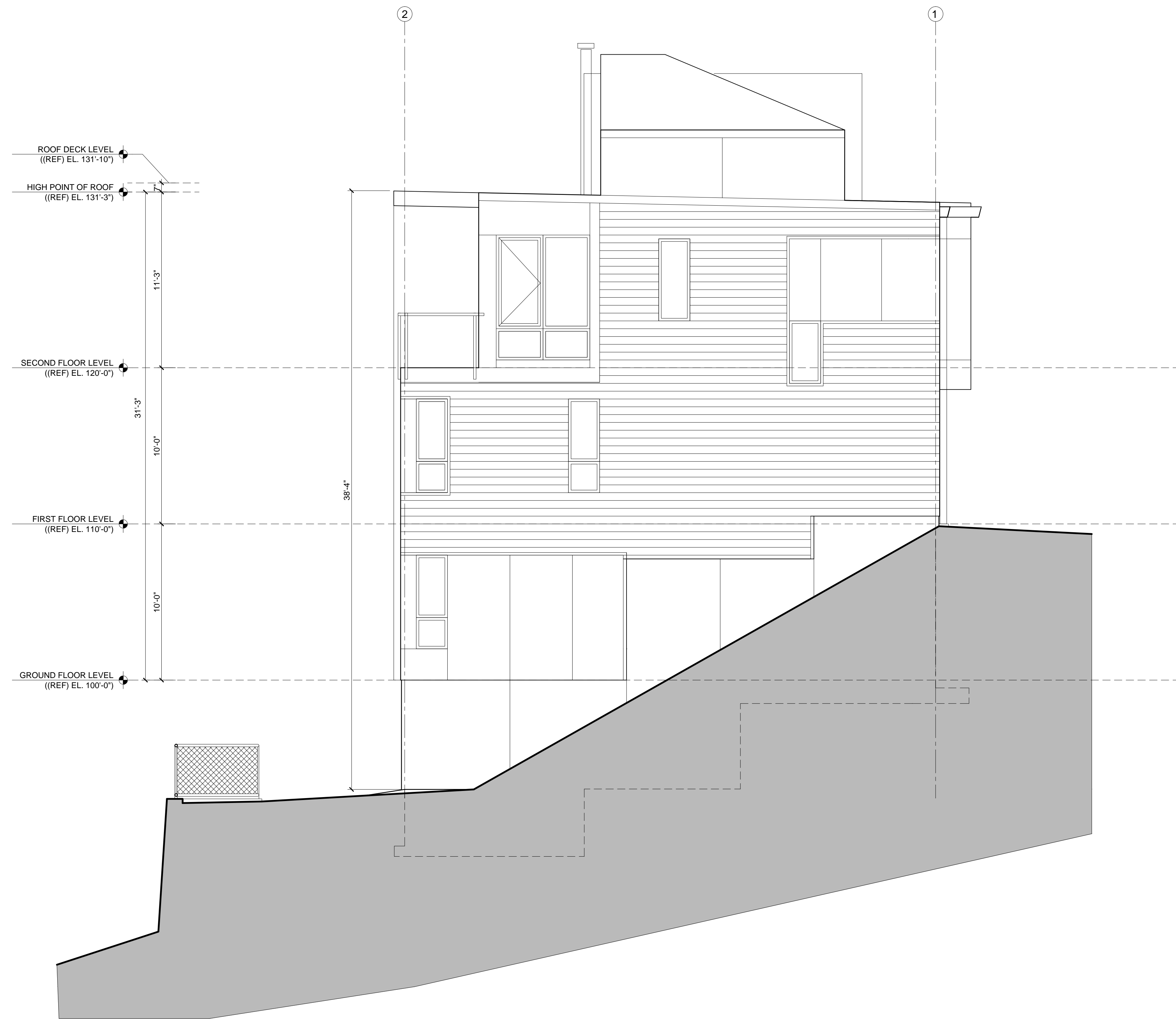
1 EAST ELEVATION 1/4"=1'-0"
