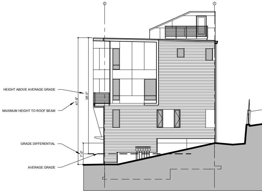
FOUR STORY BUILDING
