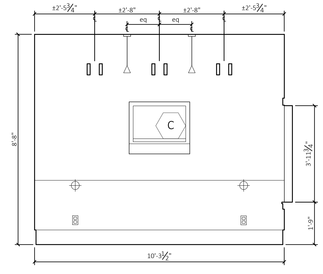
7 bedroom - south 1/2" = 1'-0"
