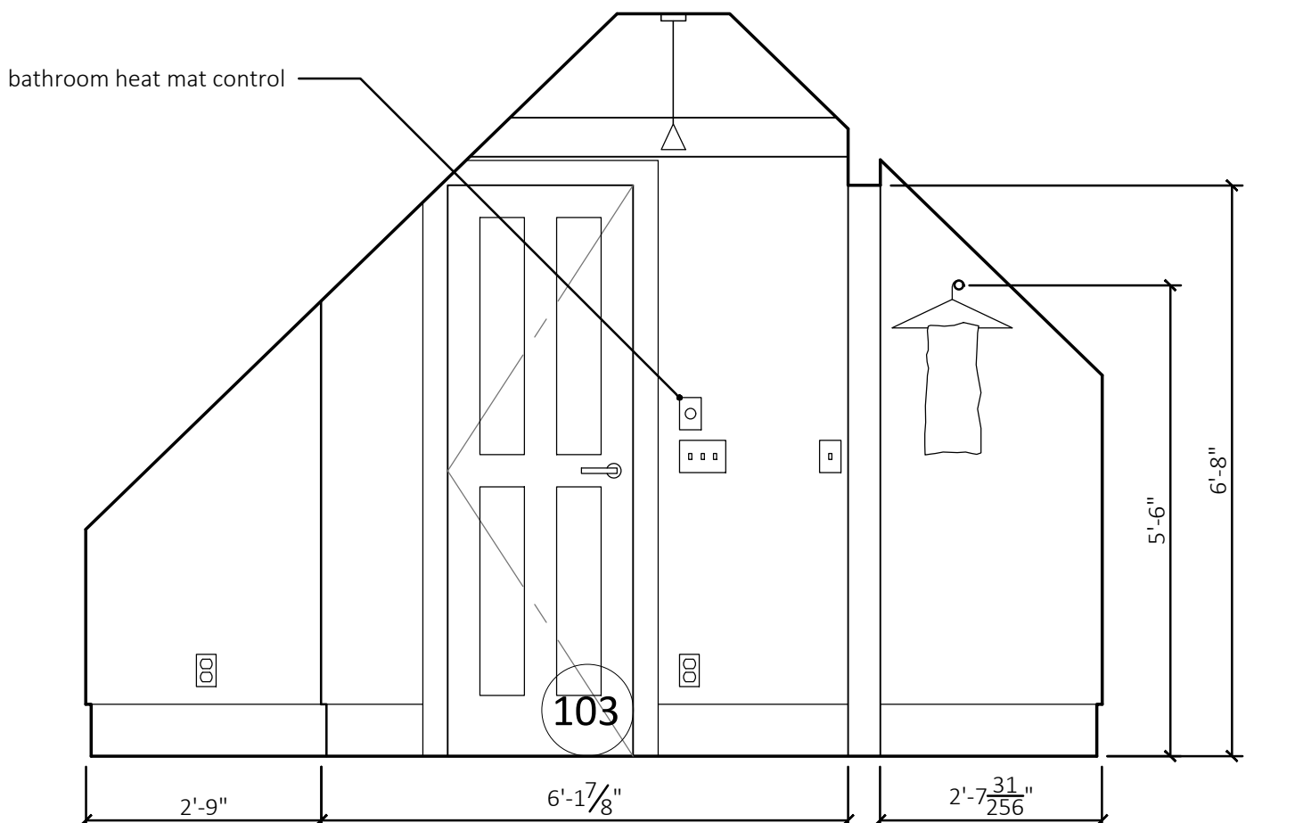
12 corridor - east 1/2" = 1'-0"
