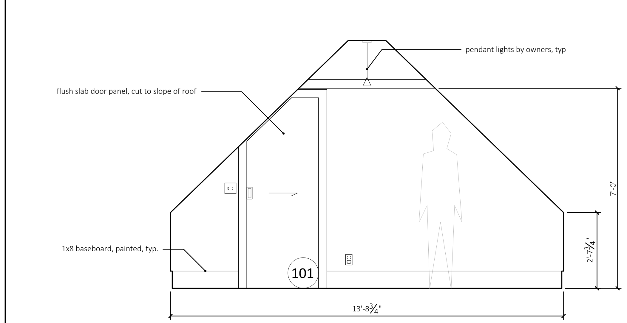
6 bedroom - east 1/2" = 1'-0"
