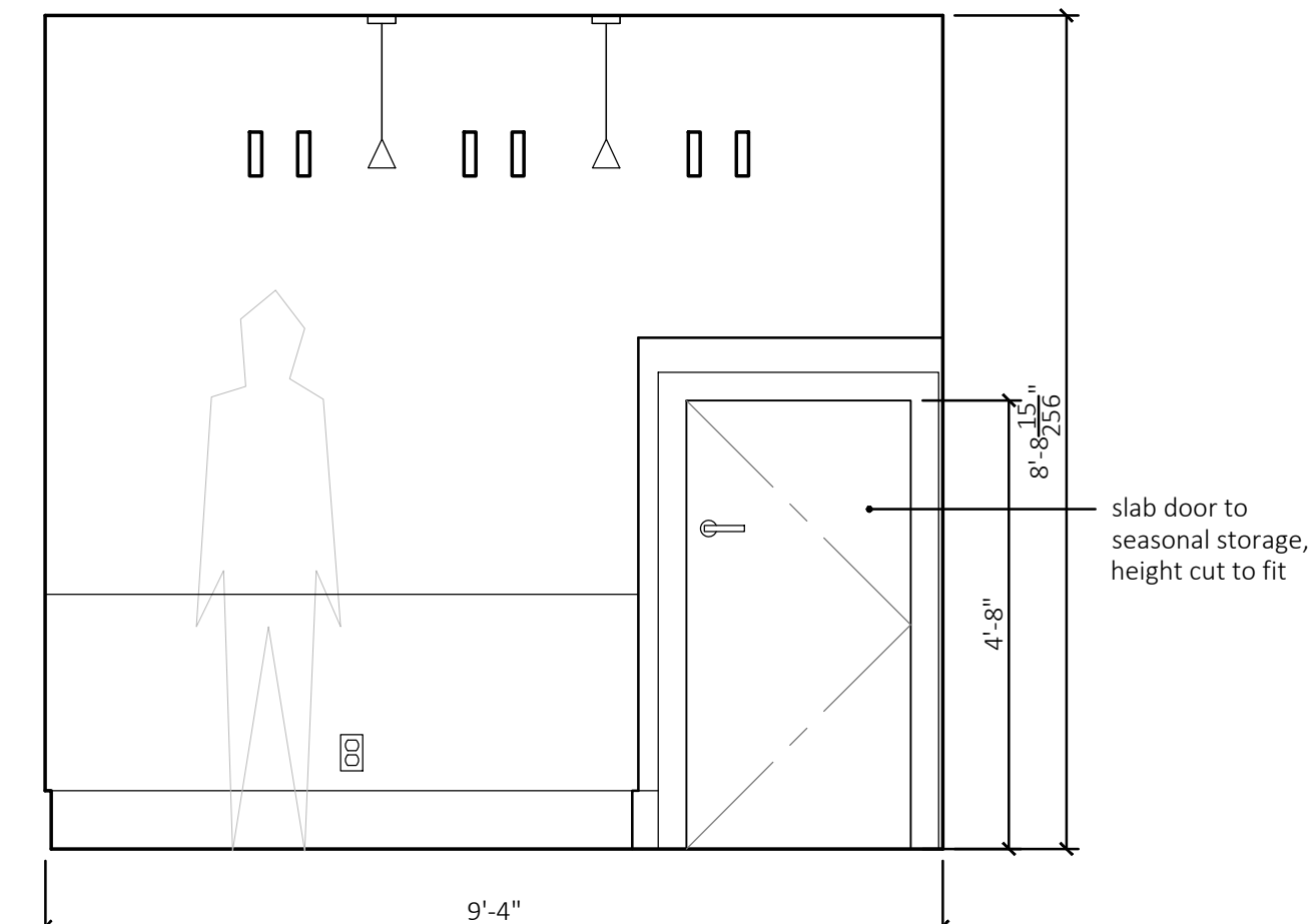
11 corridor - north 1/2" = 1'-0"
