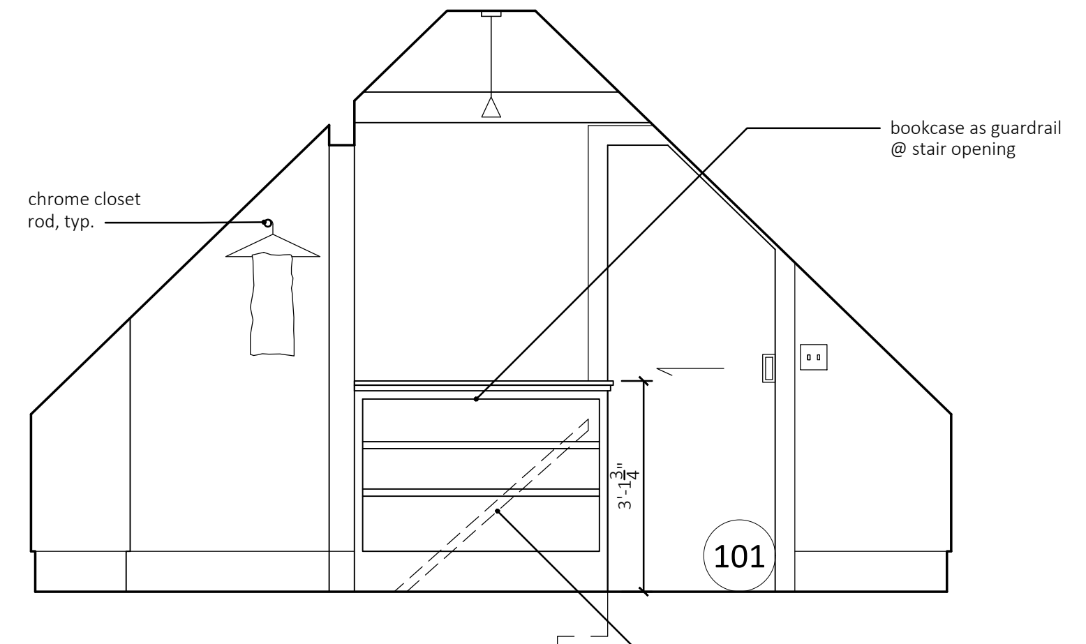
10 corridor - west 1/2" = 1'-0"
