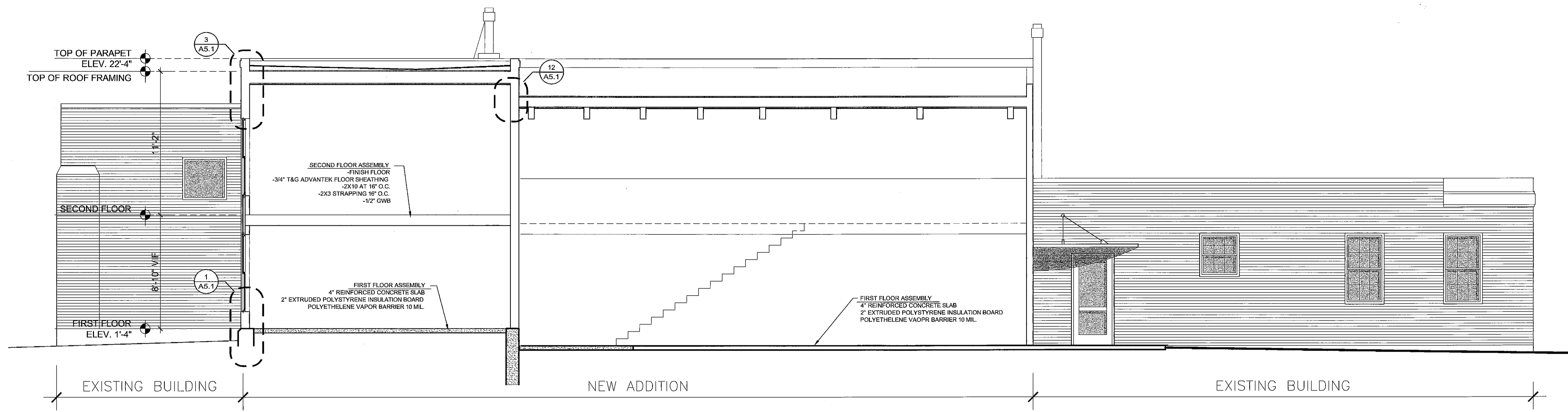
2 BUILDING SECTION A3.1 1/4" = 1'-0"
