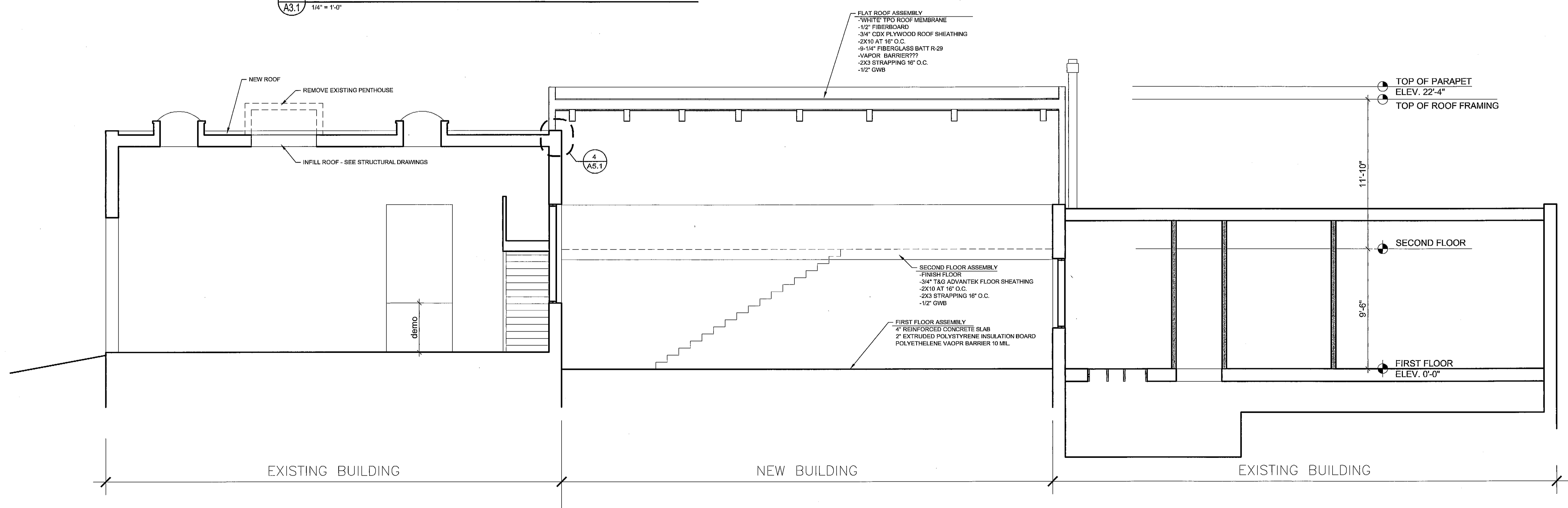
1 BUILDING SECTION A3.1 1/4" = 1'-0"
