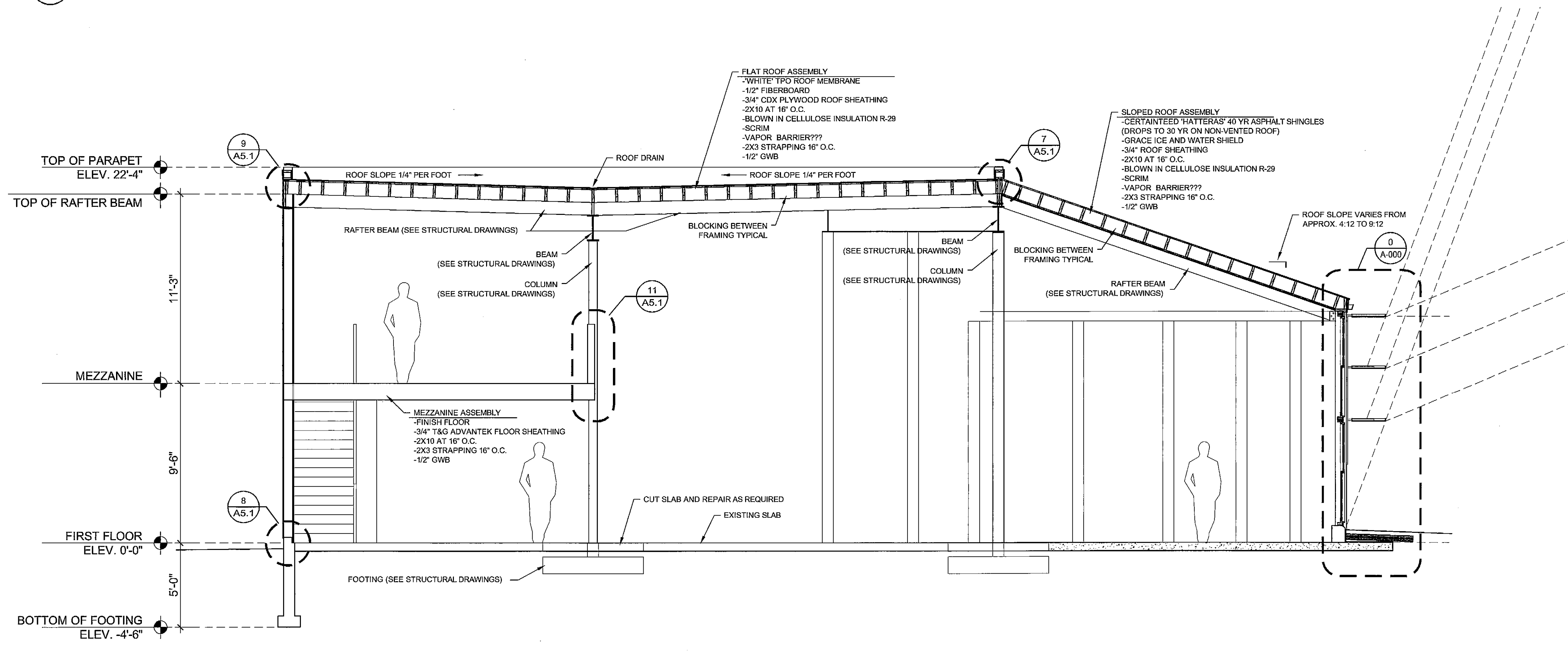
1 BUILDING SECTION THROUGH ADDITION / MEZZANINE A3.1 1/4" = 1'-0"
