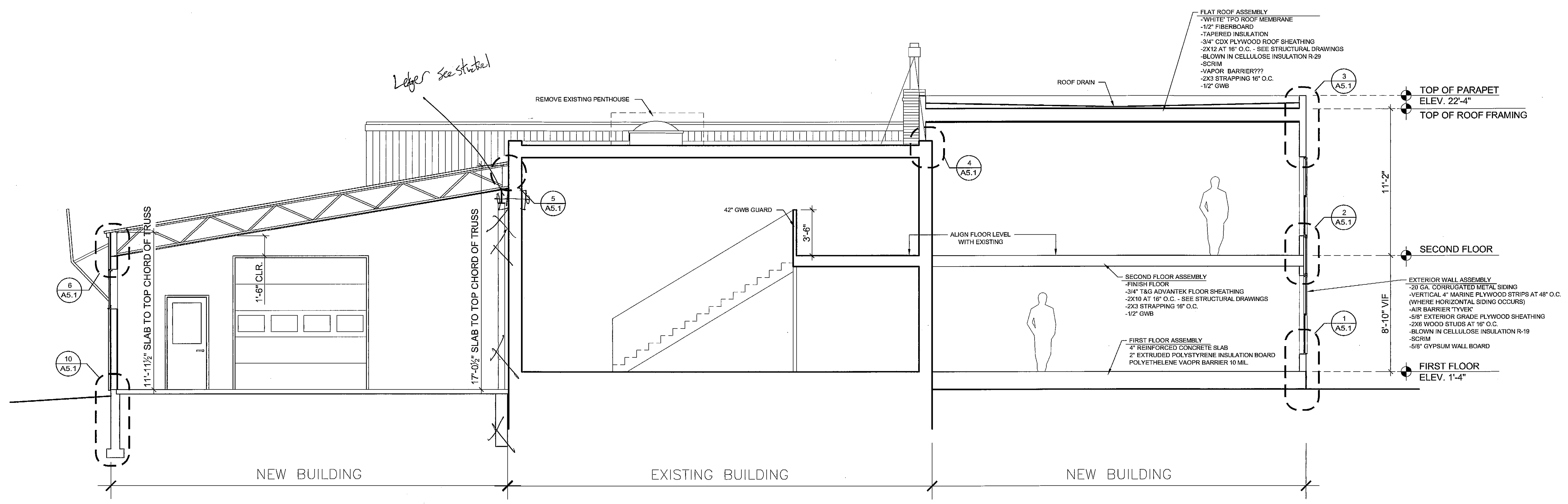
2 BUILDING SECTION THROUGH TWO STORY ADDITION / SHED ADDITION A3.1 1/4" = 1'-0"
