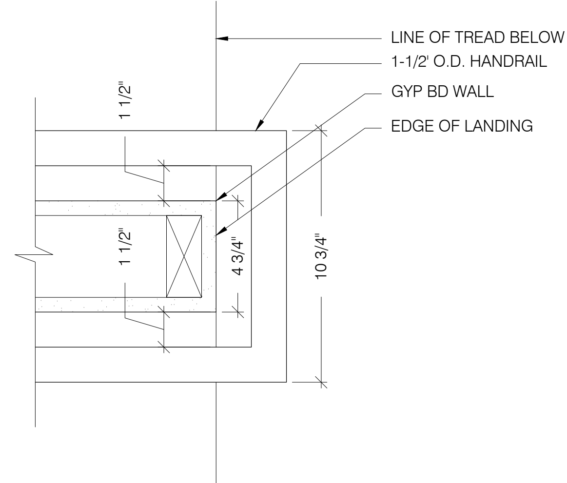
3 HANDRAIL SWITCHBACK DETAIL SCALE: 3" = 1'-0"
