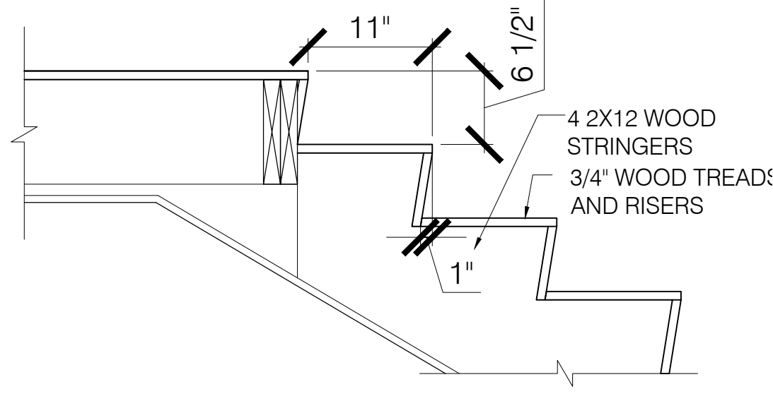
1 RISER/TREAD DETAIL - TYP. SCALE: 1" = 1'-0"
