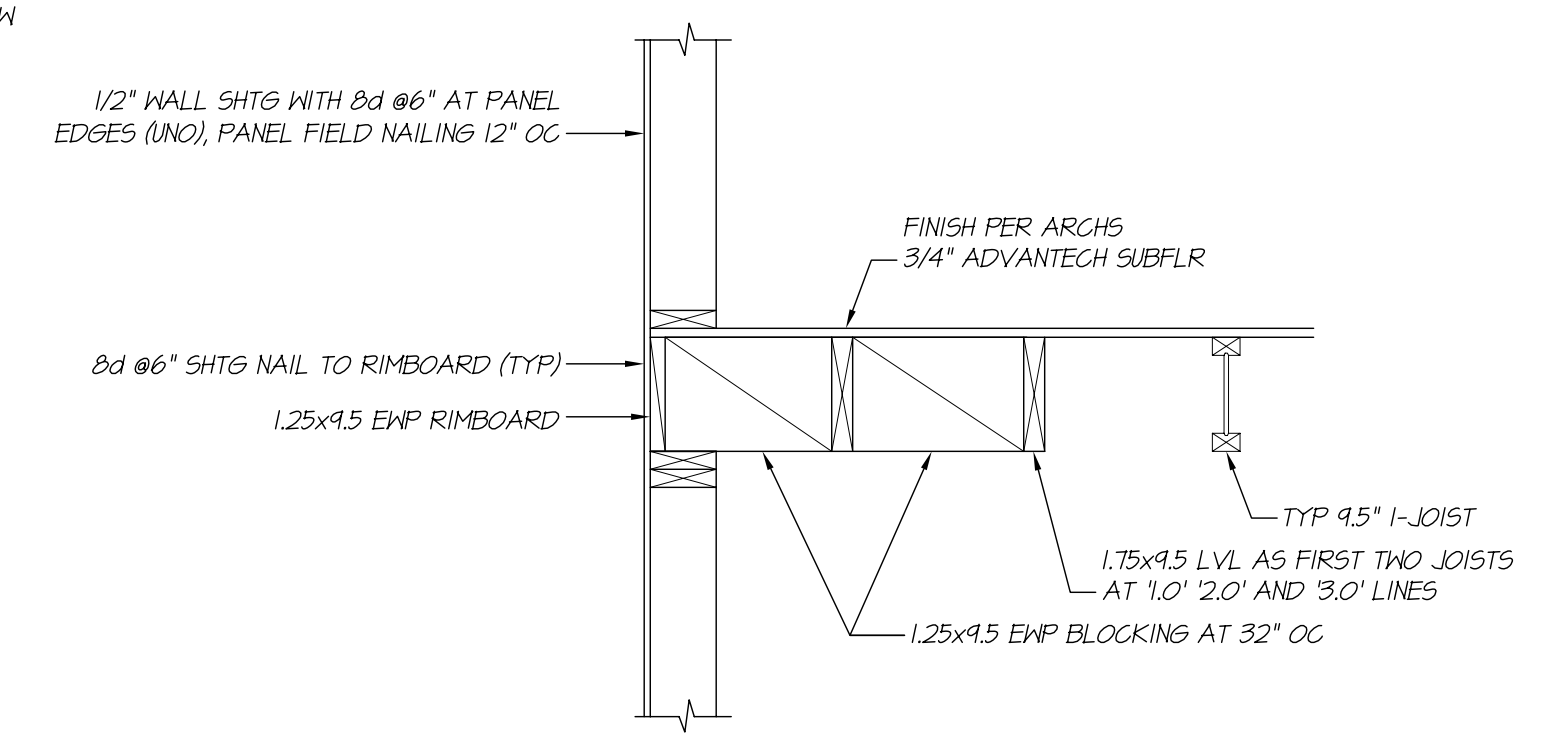
SECTION 30 3/4" = 1'-0"
