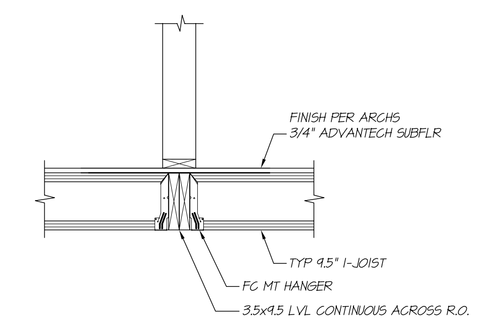
SECTION 32 3/4" = 1'-0"
