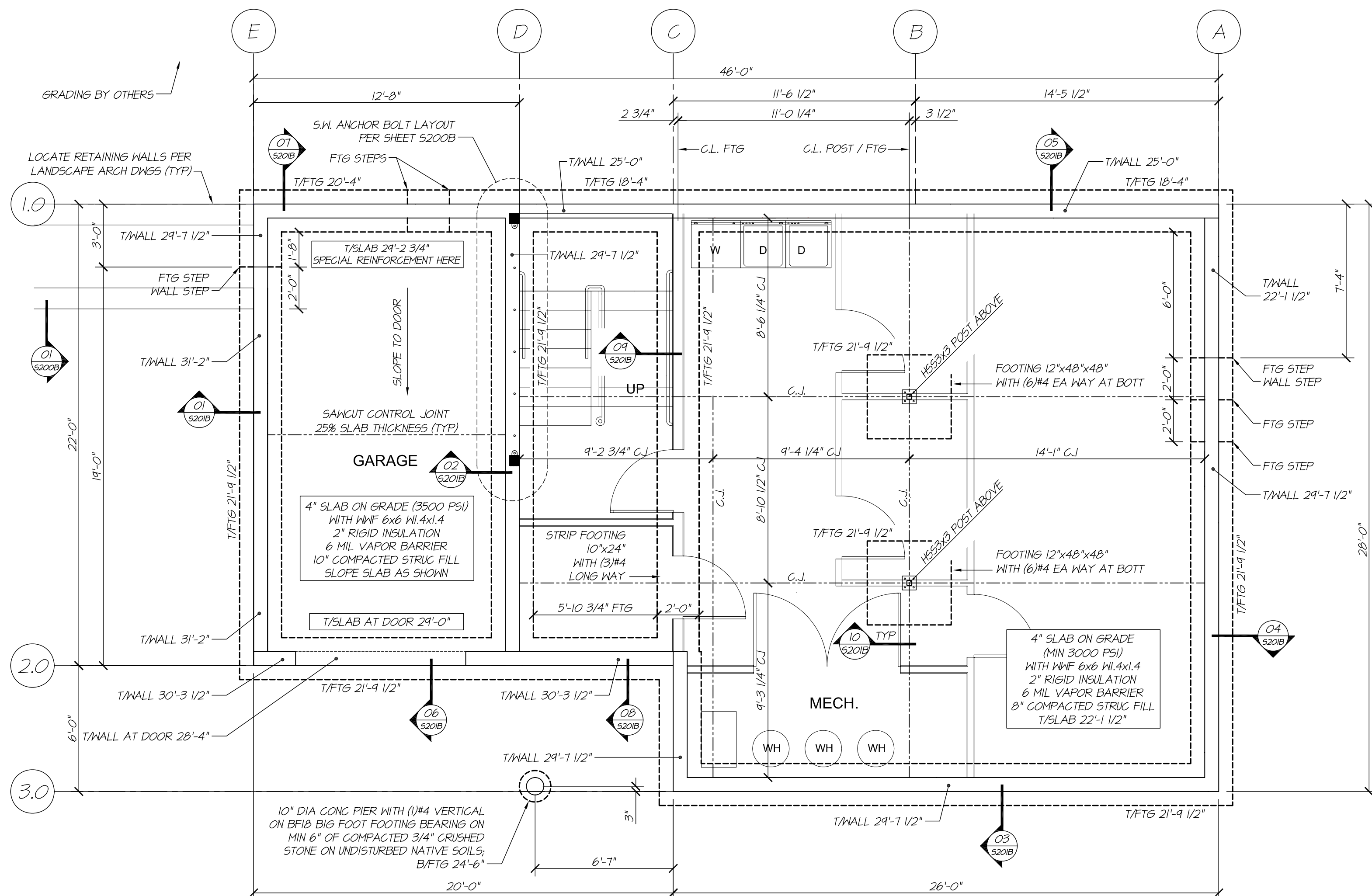
FOUNDATION PLAN 1/4" = 1'-0"
