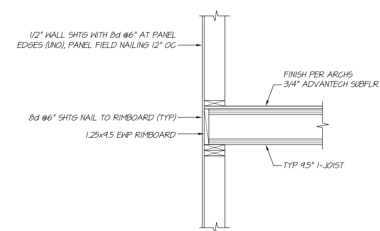
SECTION 31 3/4" = 1'-0"
