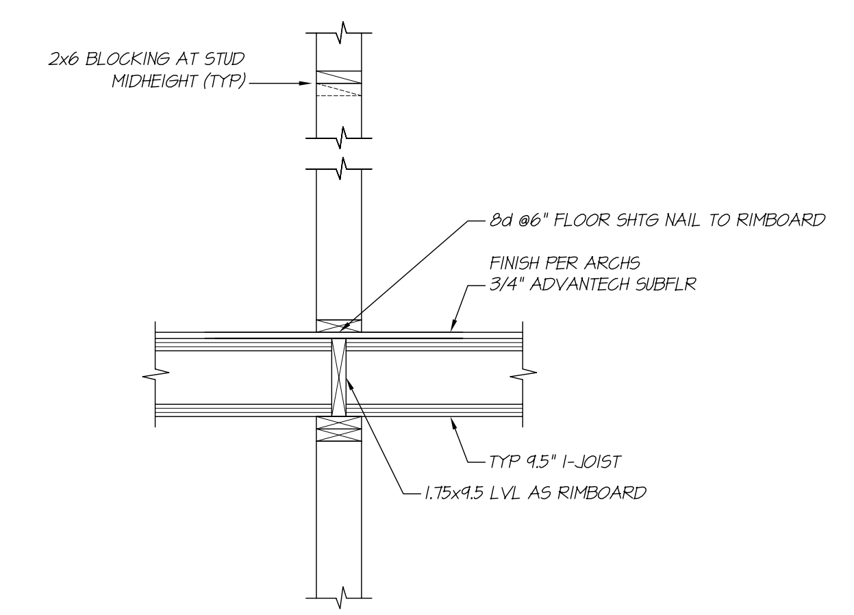
SECTION 33 3/4" = 1'-0"
