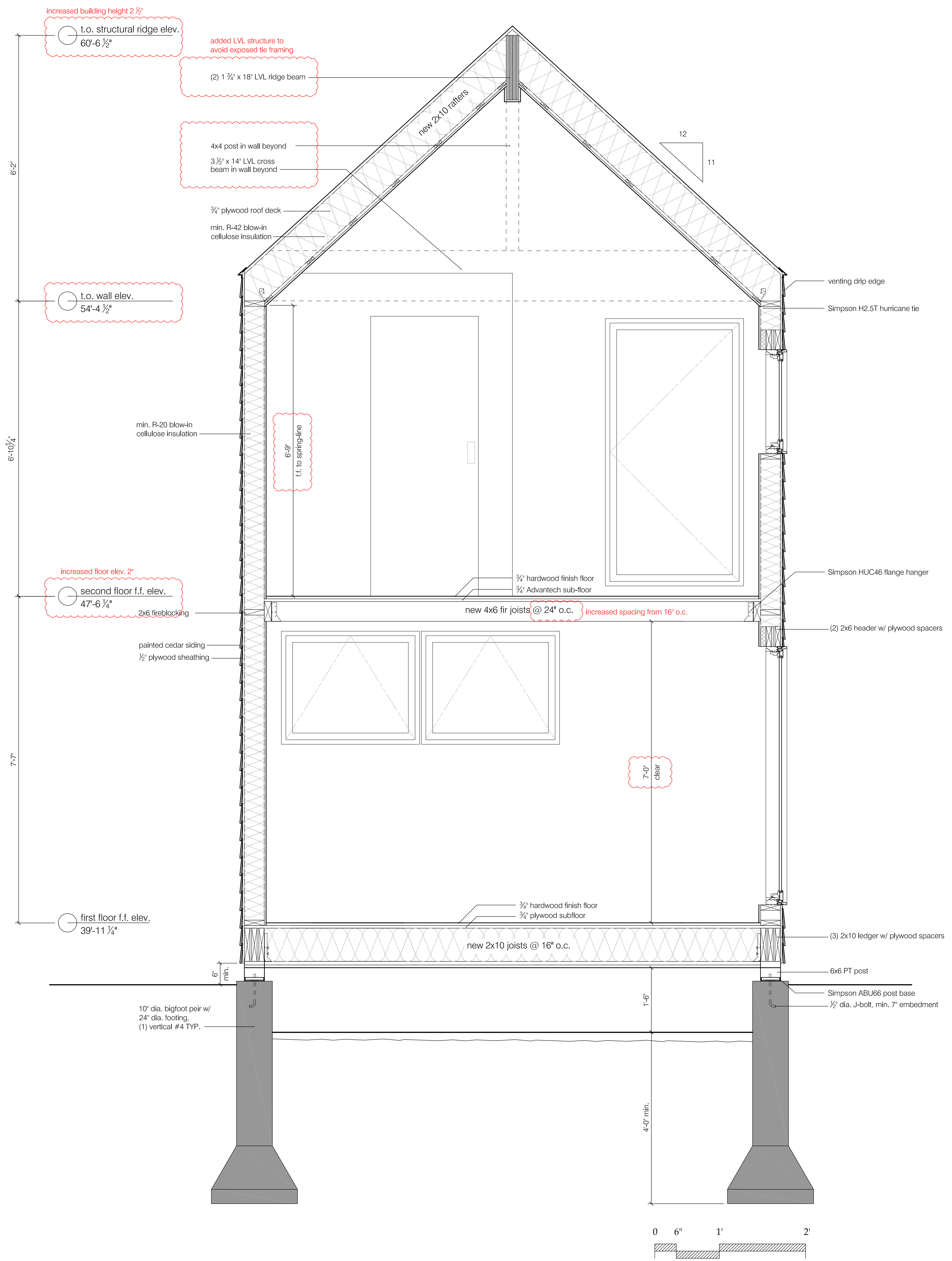
1 building section @ existing portion 3/4" = 1'-0"
