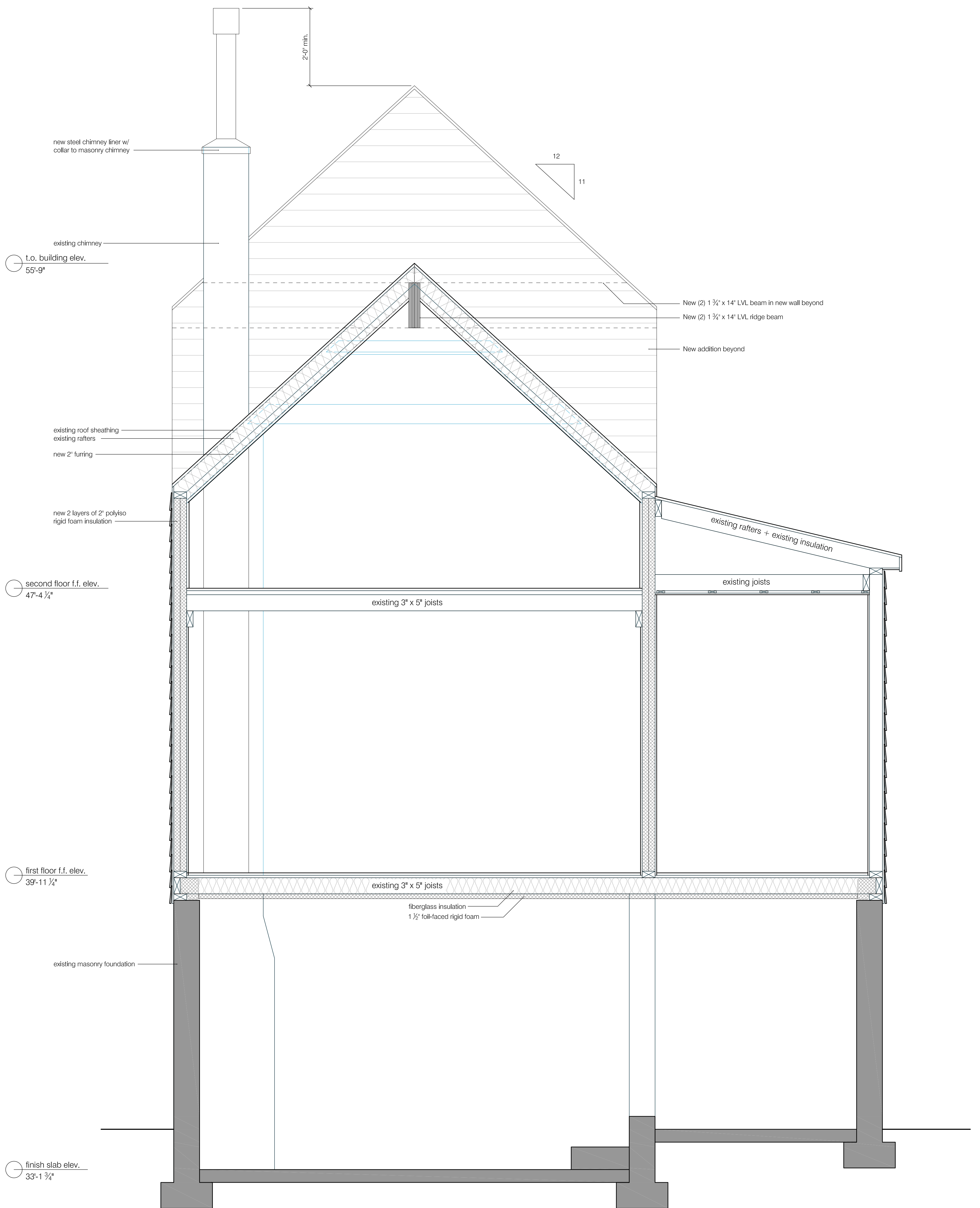
1 building section @ existing structure 3/4" = 1'-0"
