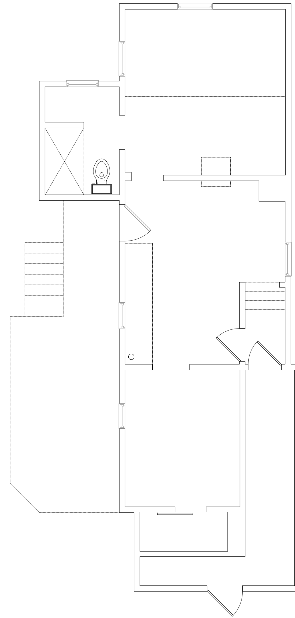
2 first floor plan \frac{1}{4}'' = 1'-0''
