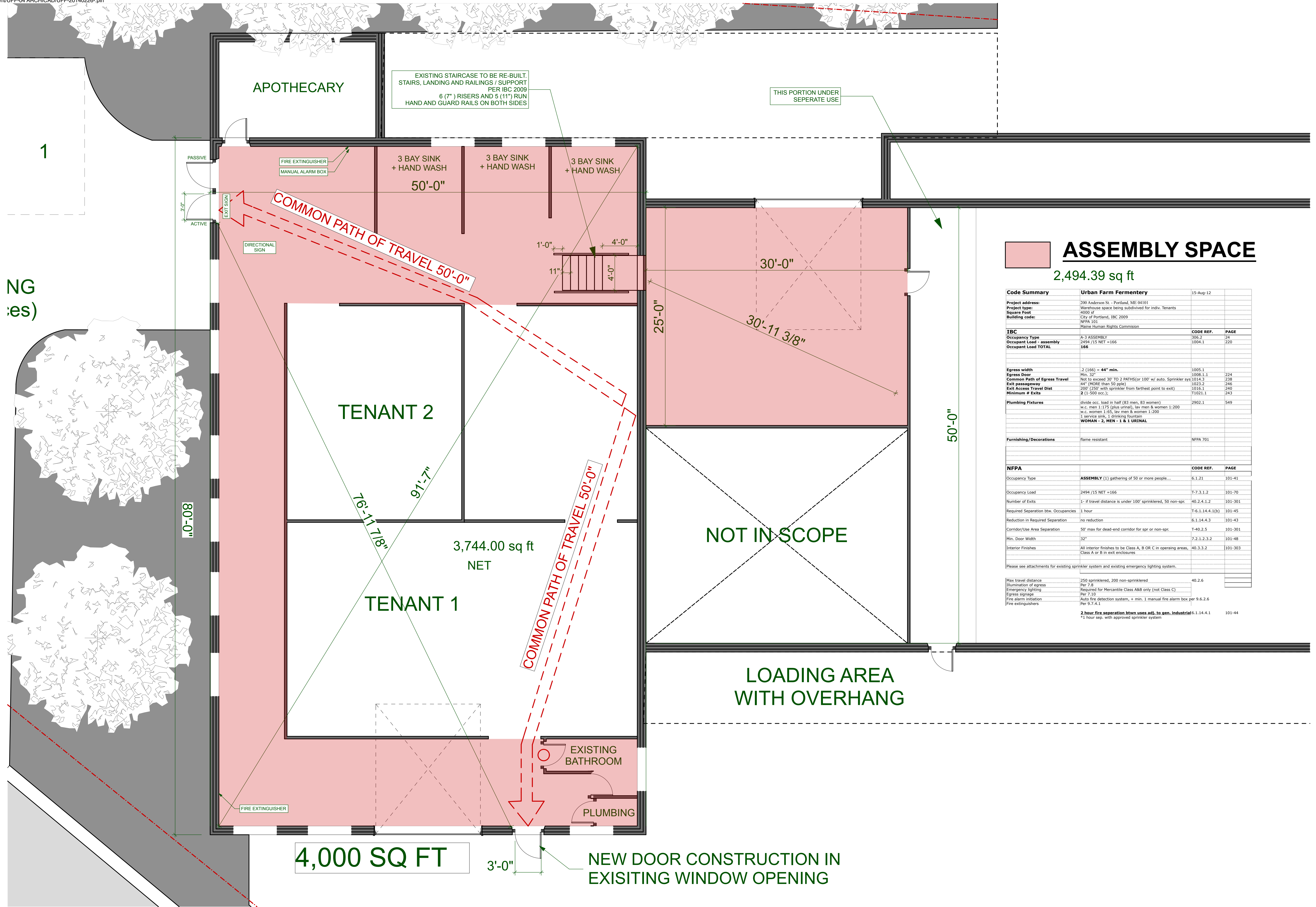
1 MAIN LEVEL A-0.1 SCALE: 3/16" = 1'-0"
