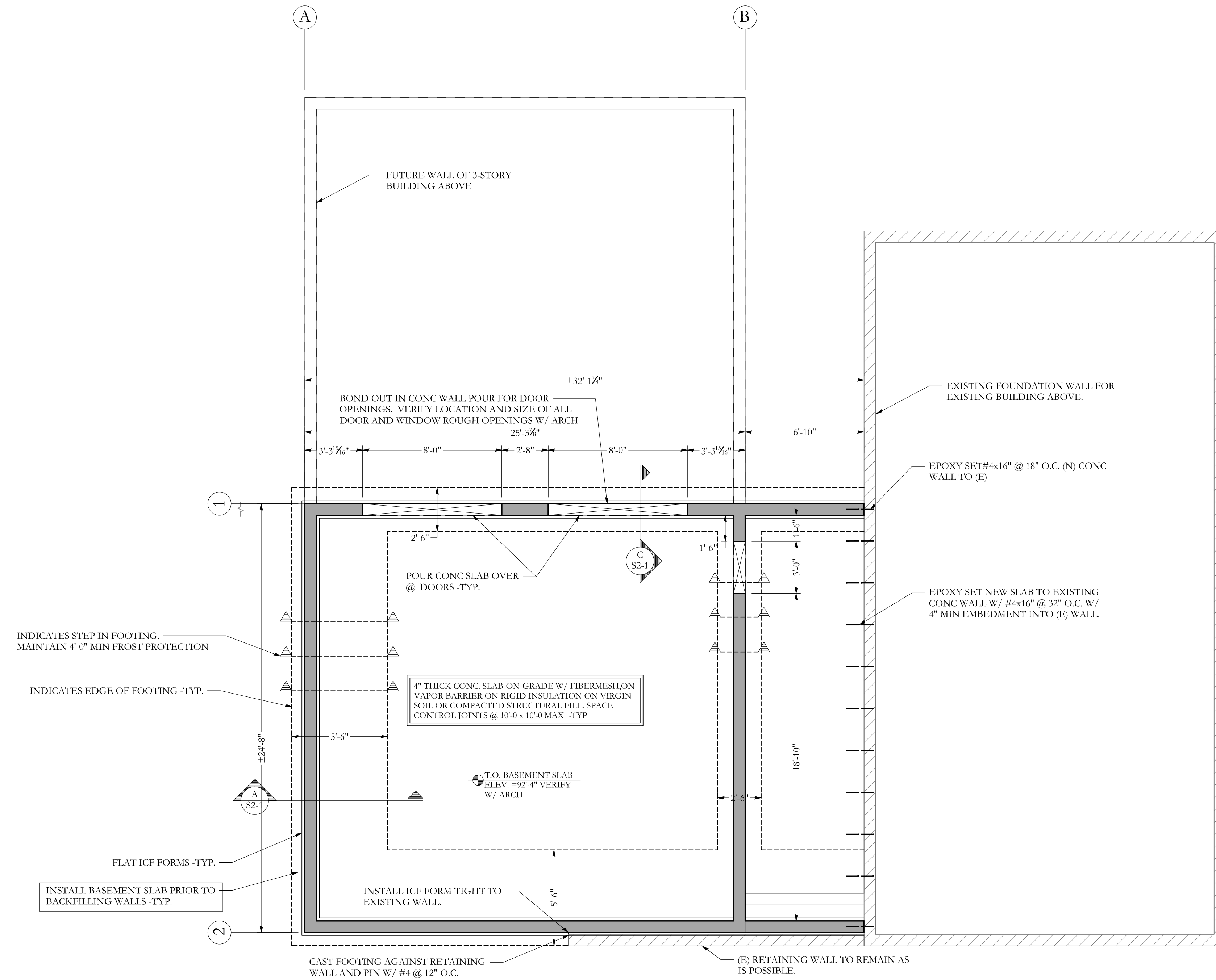
FOUNDATION/BASEMENT FLOOR PLAN SCALE 1/4"=1'-0"
