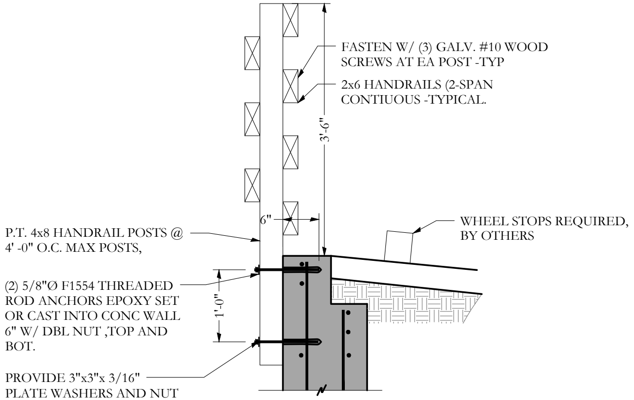
SECTION SK-2 3/4"=1'-0
