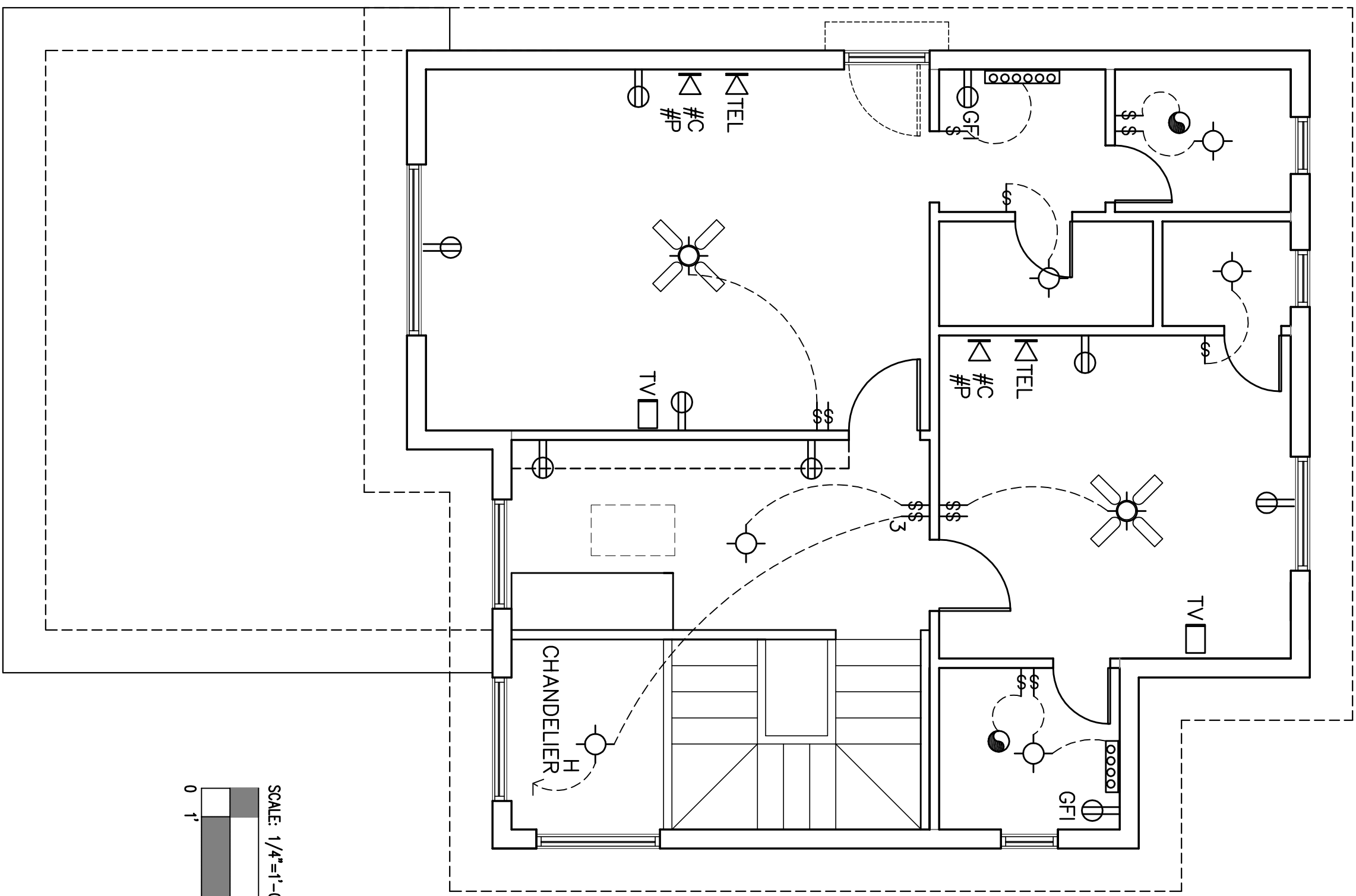
UPPER LEVEL CEILING PLAN
