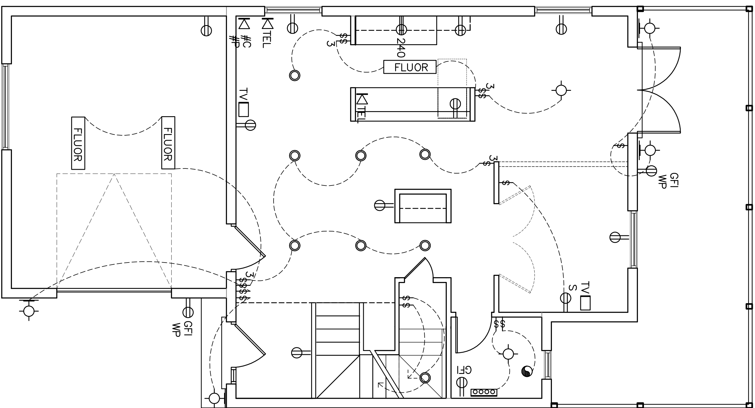
ENTRY LEVEL CEILING PLAN
