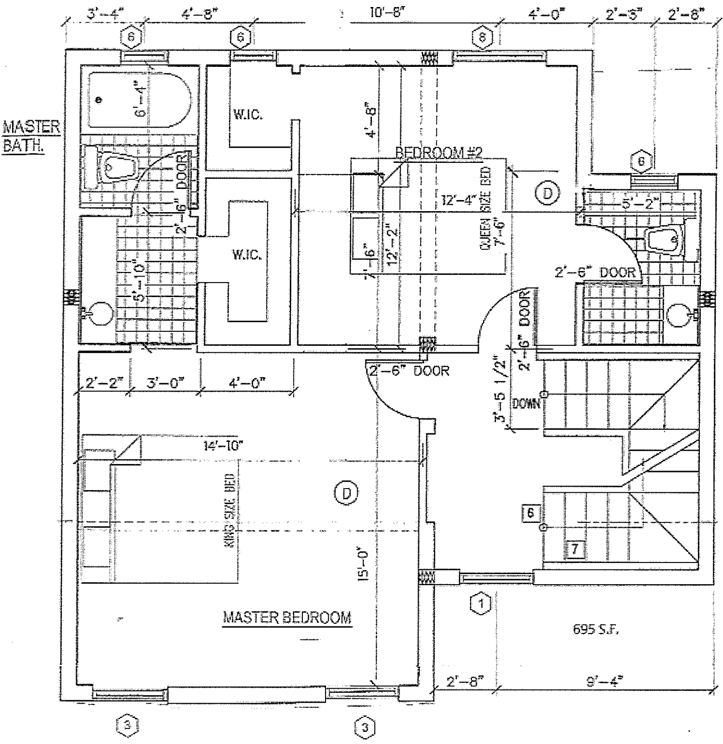
2 UPPER FLOOR PLAN 0' 4' 8'
