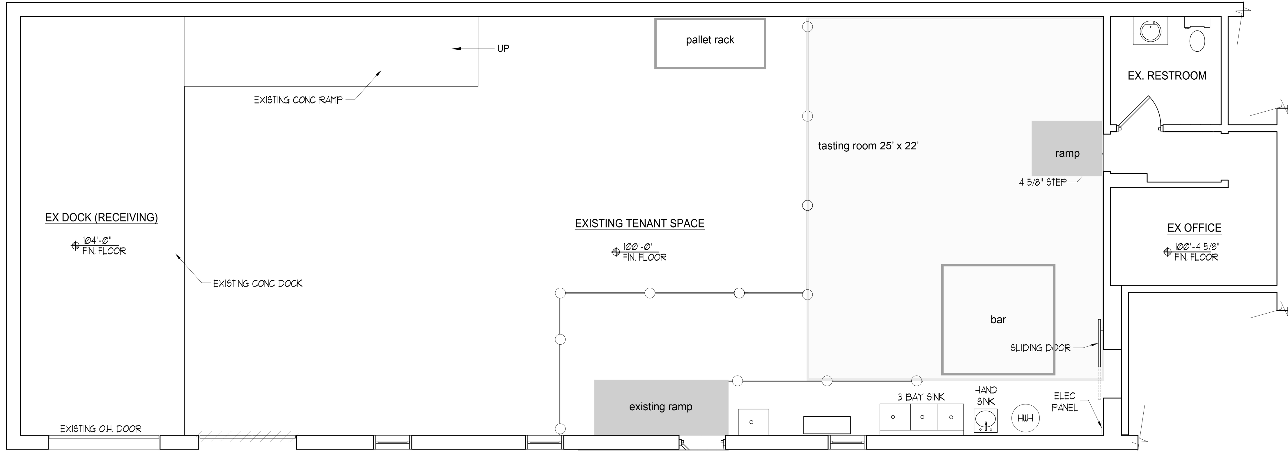
1 DEMOLITION PLAN SCALE: 1/4" = 1'-0"
