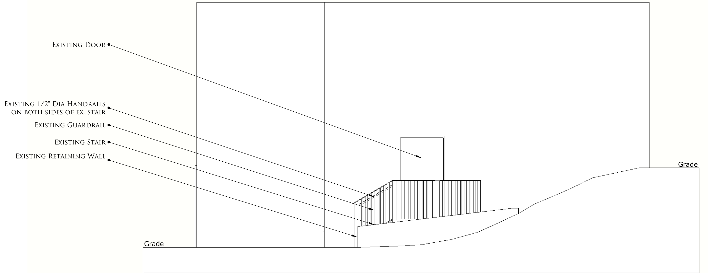
SIDE ELEVATION SCALE 1/5" = 1'
