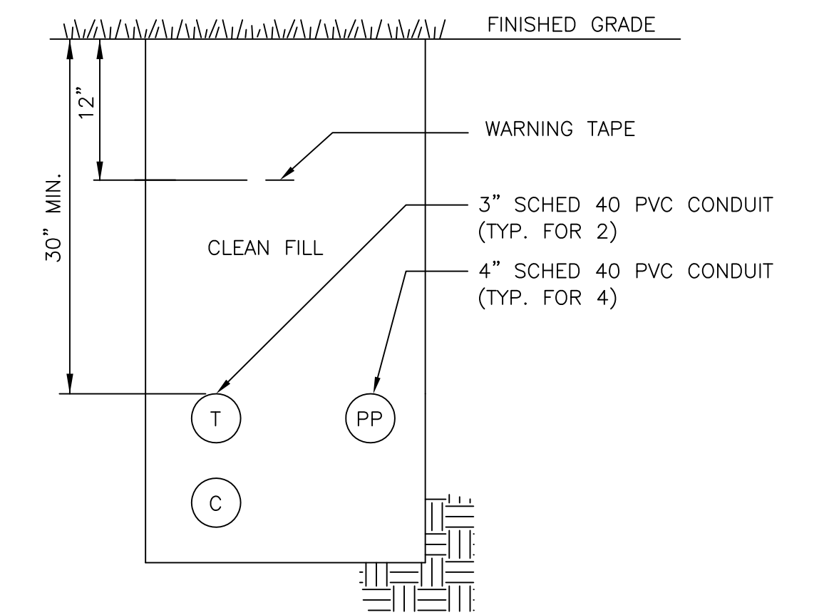
2 DUCT BANK SECTION A-A SCALE: NOT TO SCALE
