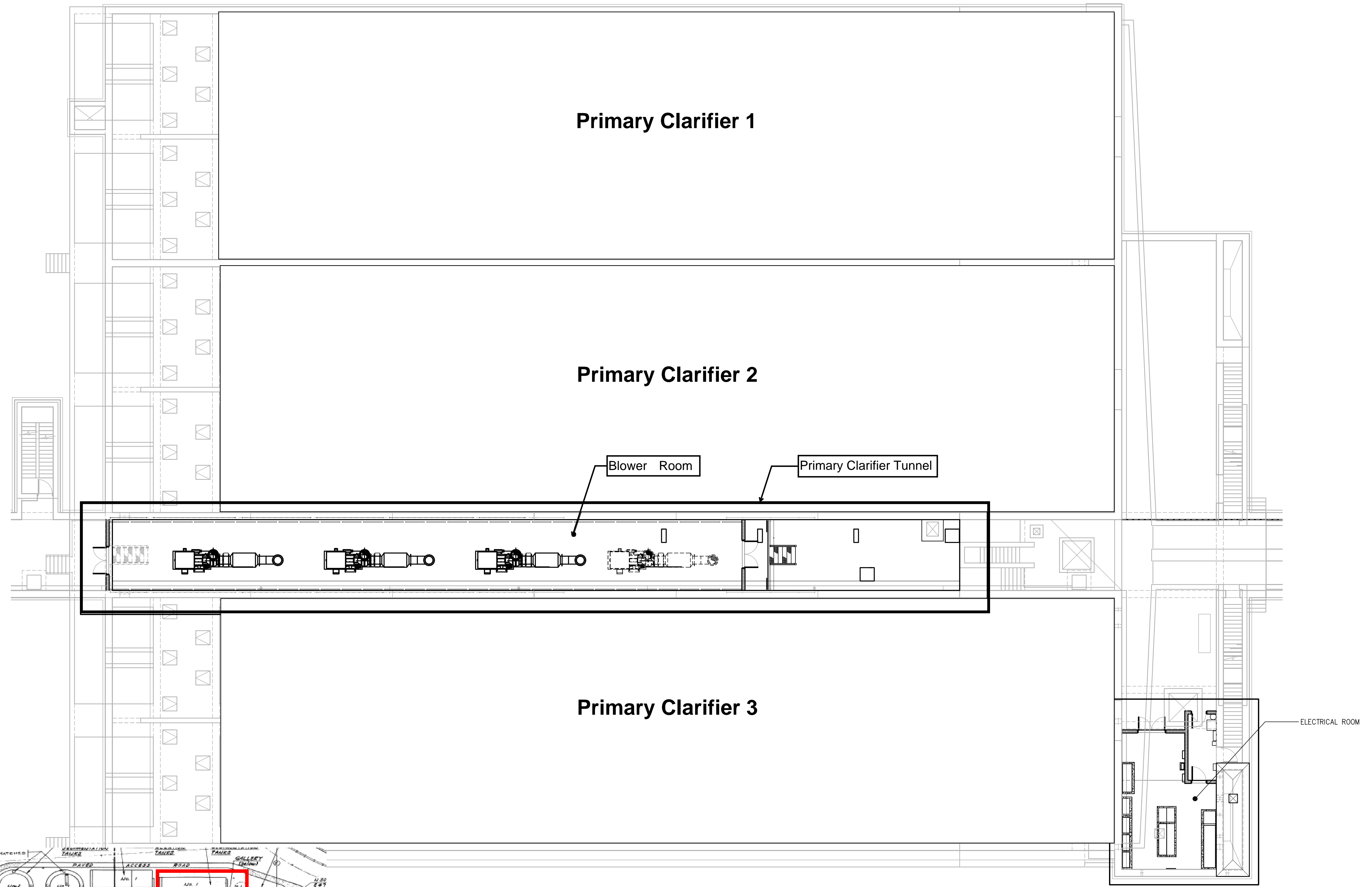
BOTTOM PLAN 3/32" = 1'-0"
