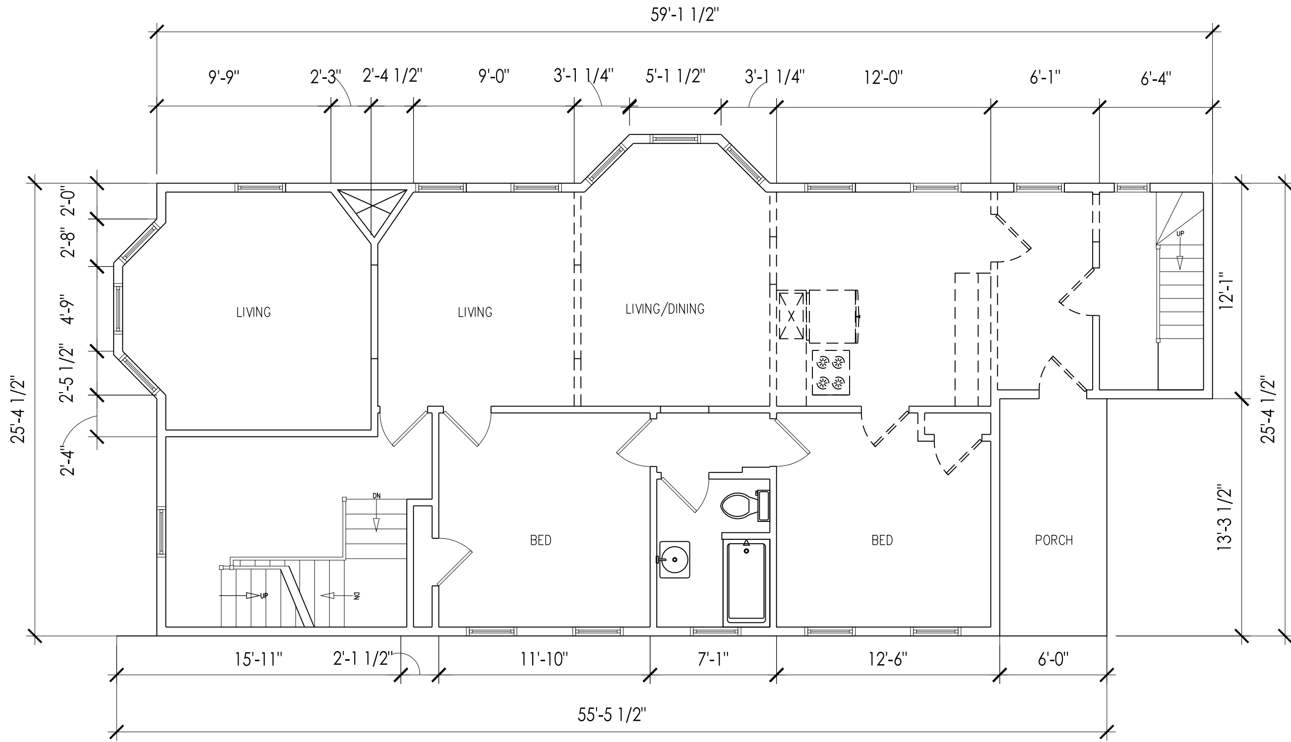
SECOND LEVEL PLAN SCALE 3/16" = 1'-0"
