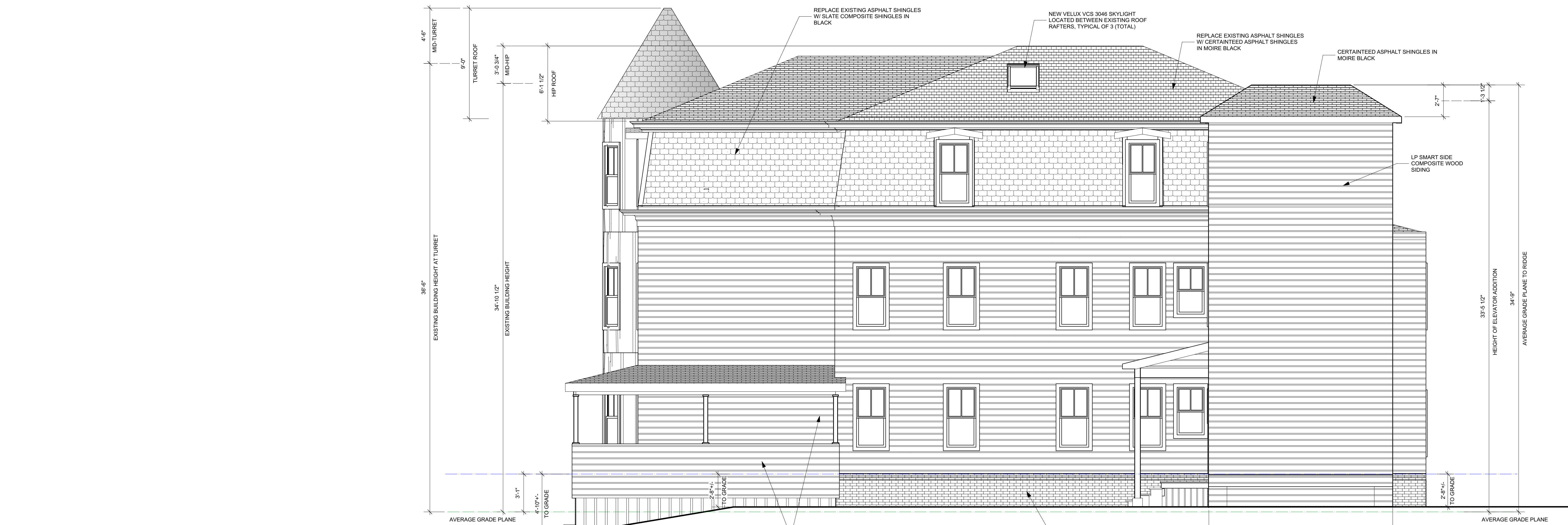
3 NORTH ELEVATION Scale: 1/4" = 1'-0"
