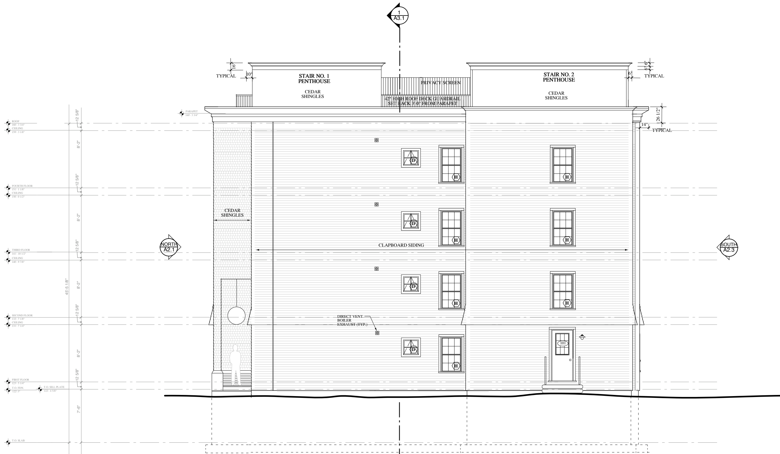
1 WEST ELEVATION SCALE: 1/4" = 1'-0"
