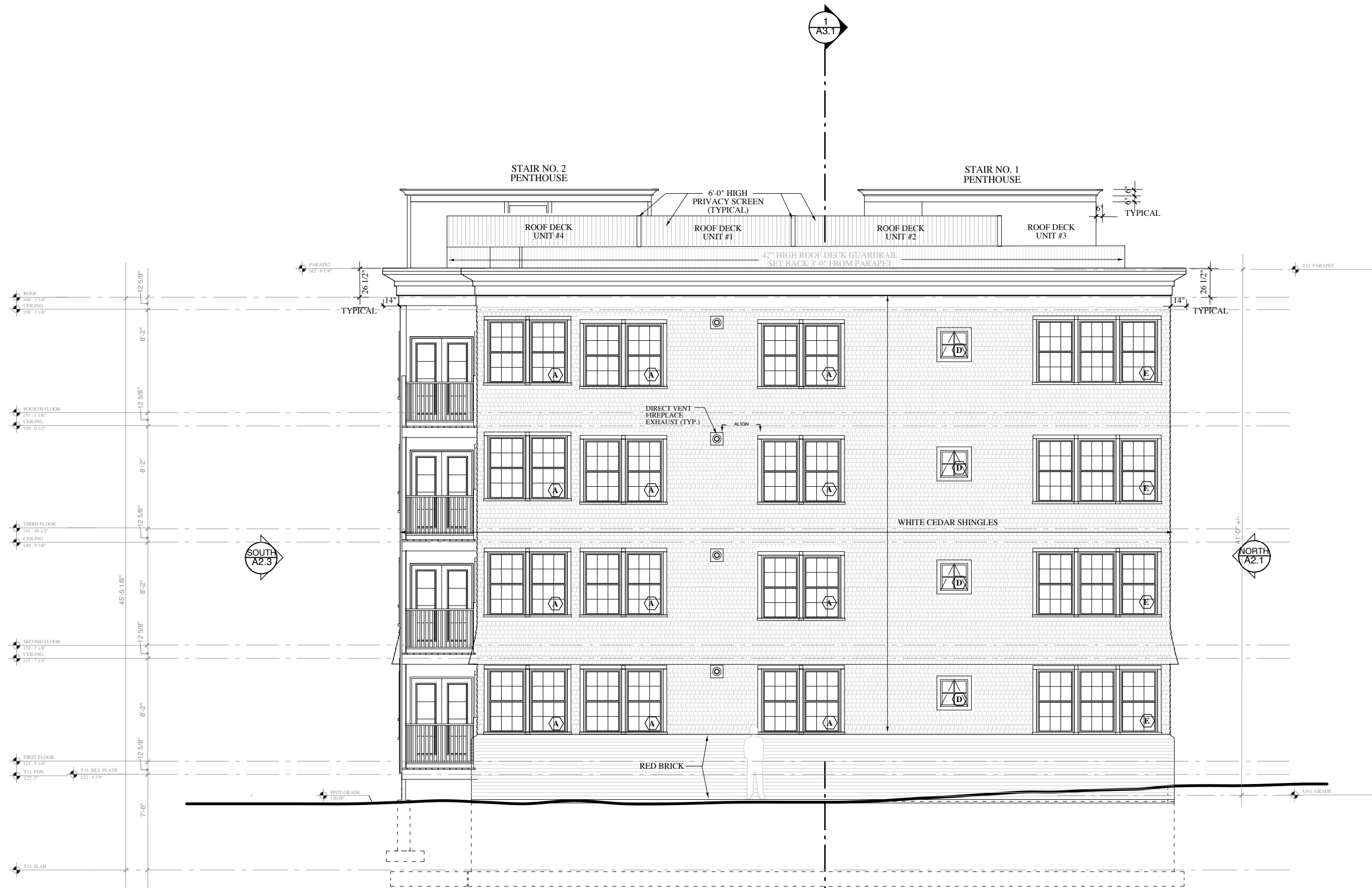
1 EAST ELEVATION SCALE: 1/4" = 1'-0"
