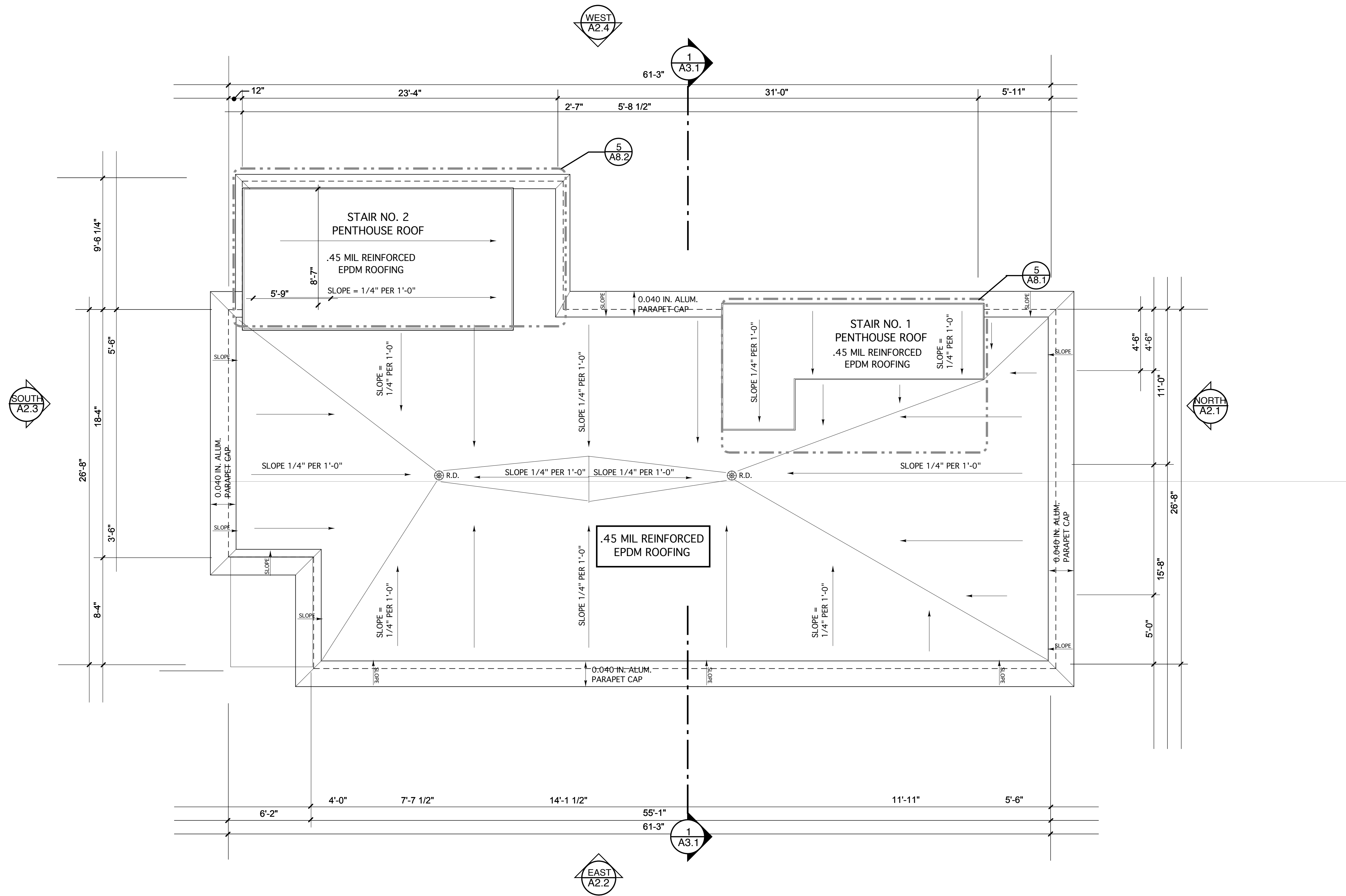
1 ROOF PLAN SCALE: 1/4" = 1'-0"
