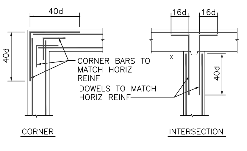
TYP WALL AND SLAB REINF DETAILS (U.O.N.) N.T.S.
