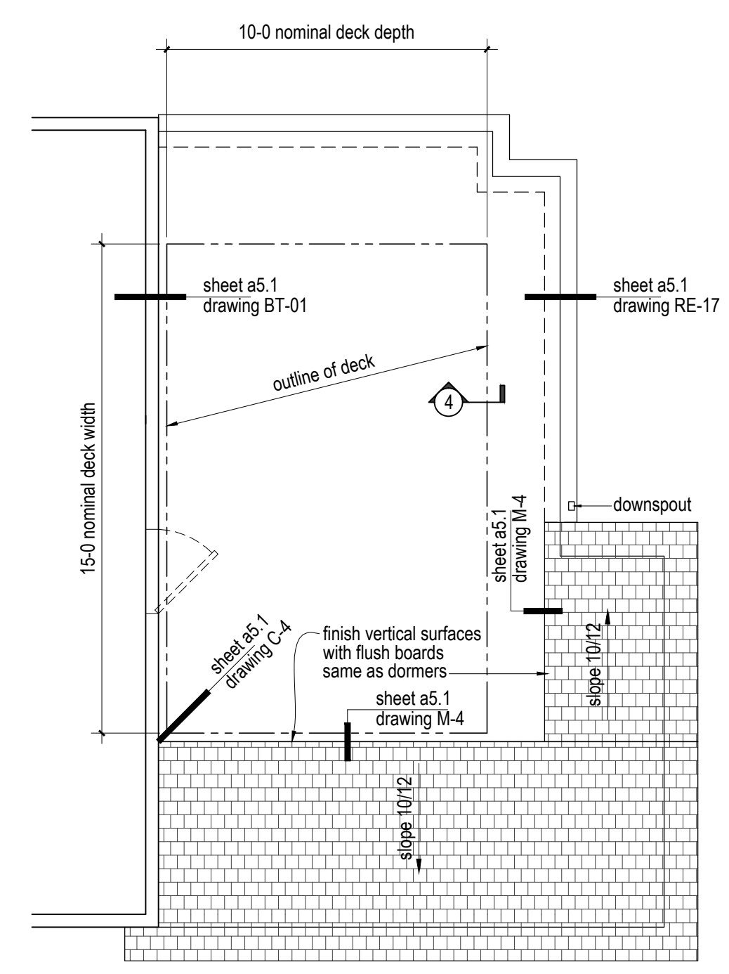
3rd floor roof plan 1/4"=1'-0"
