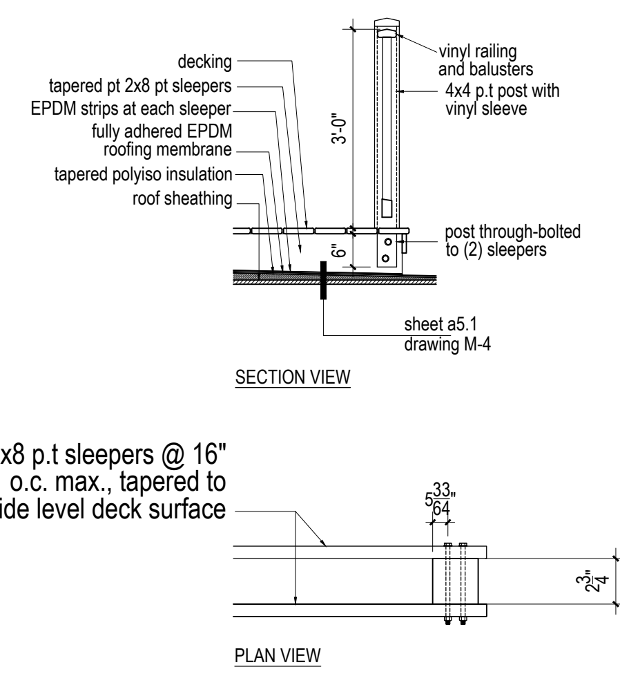
A Roof Deck Railing Detail 1/2"=1'-0"
