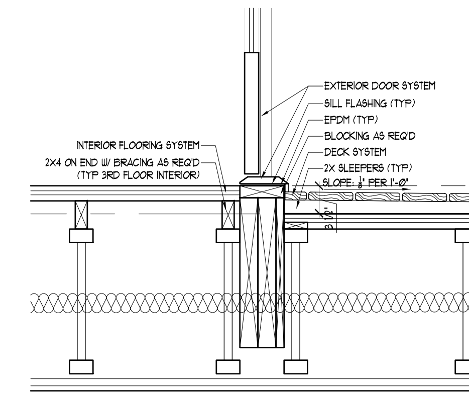
3 ROOF DECK AND THRESHOLD DETAIL
