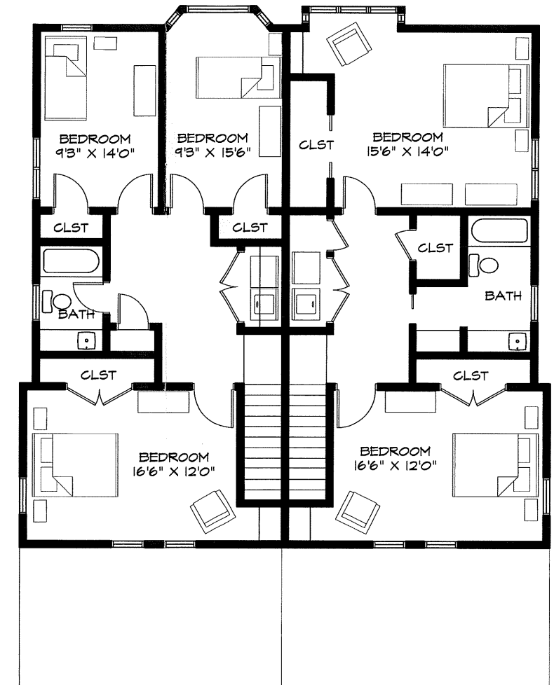
THIRD FLOOR PLAN 3 BR - Scheme A
