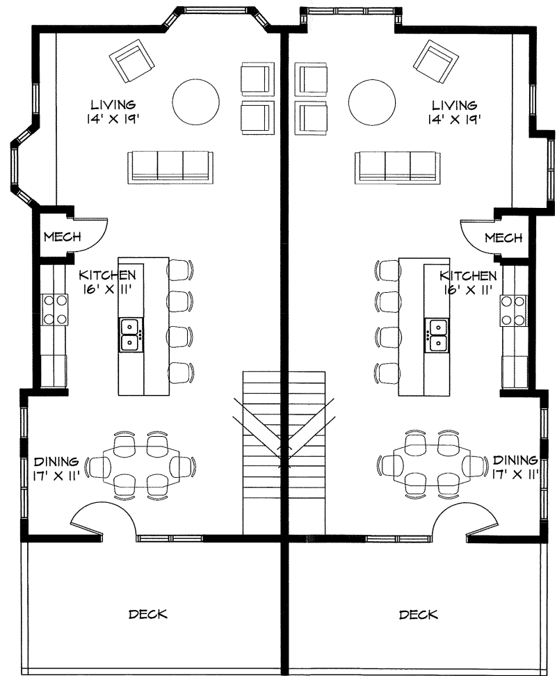
SECOND FLOOR PLAN 3 BR - Scheme B
