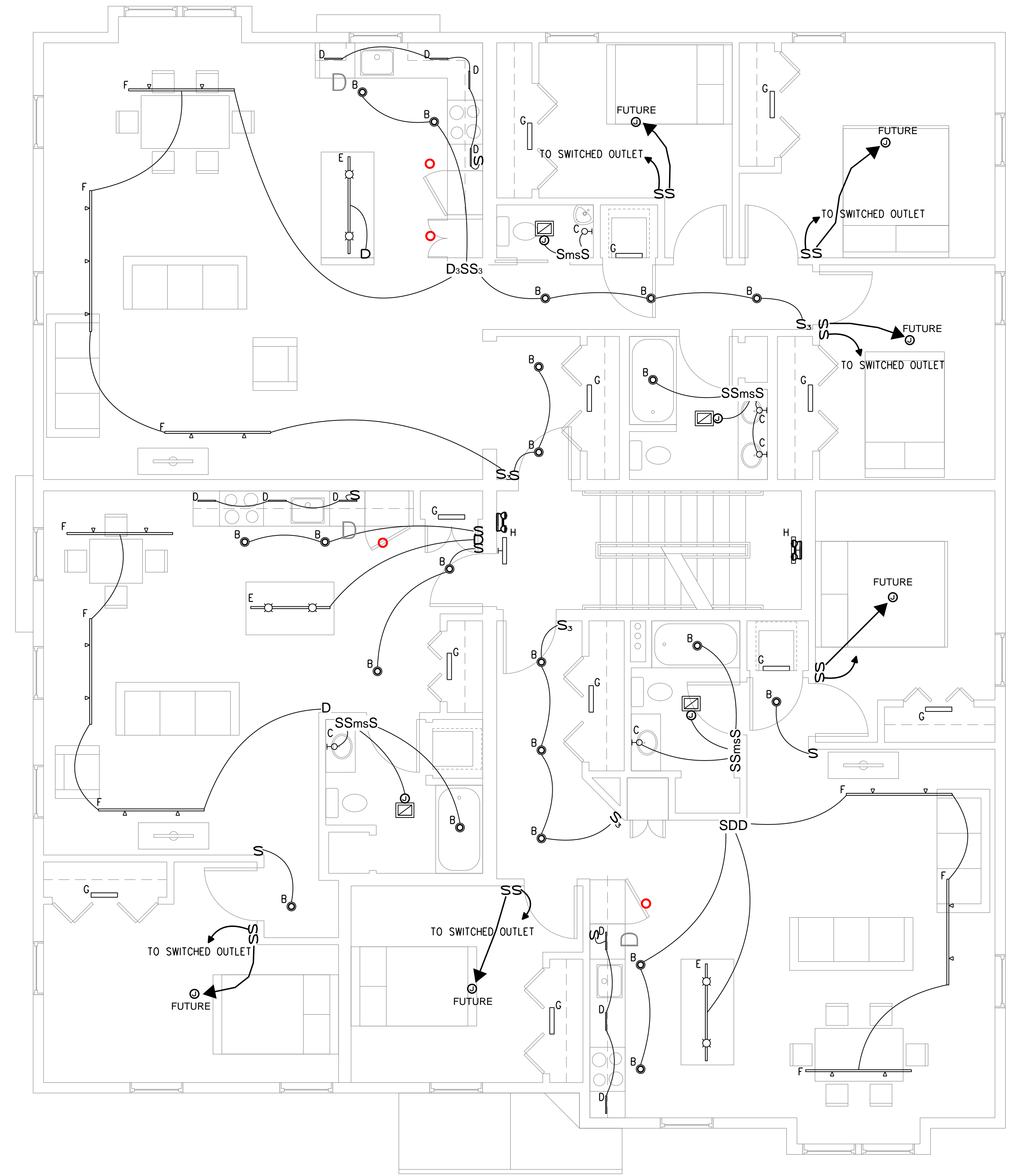
TYPICAL SECOND & THIRD FLOOR LIGHTING PLAN SCALE: 1/4" = 1'-0"
