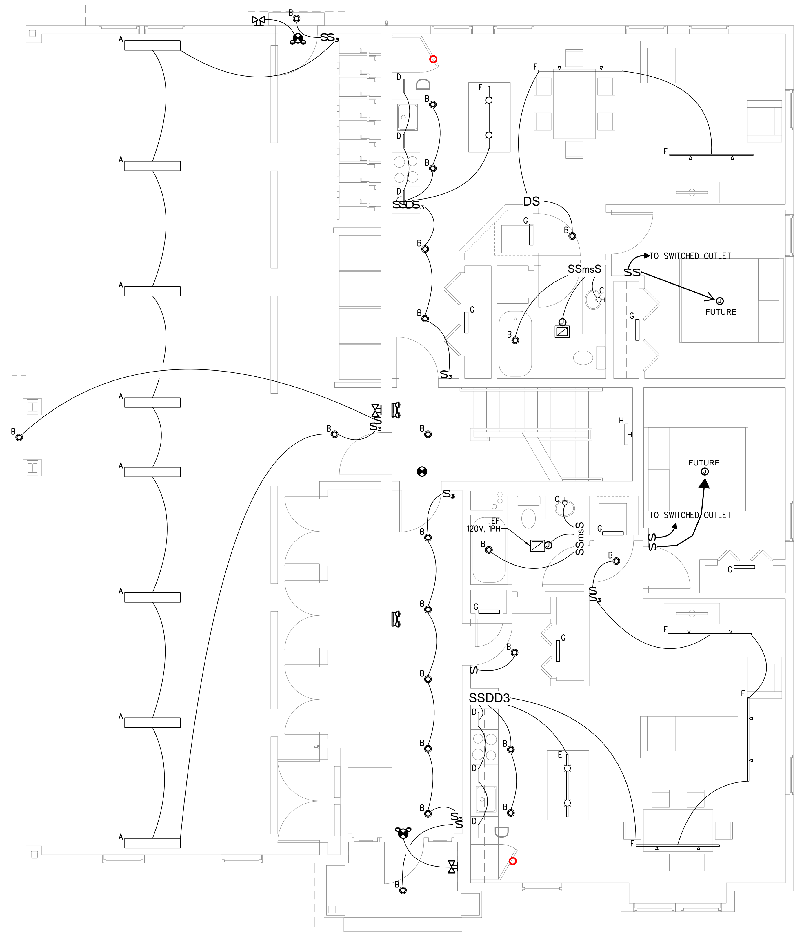
FIRST FLOOR LIGHTING PLAN SCALE: 1/4" = 1'-0"
