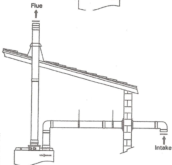
Two pipe system (room air independent) hybrid
